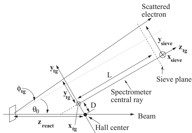
FIG. 12. Top view of the TCS (x_{tg}, y_{tg}, z_{tg}) and the sieve plane coordinate system (x_{sieve}, y_{sieve}) . The z_{tg} axis is along the HRS central ray, the y_{tg} axis is pointing to the left, the x_{tg} axis is pointing vertically down, and the origin of the TCS is the point along the HRS central ray that is the closest to the Hall center. The \phi_{tg} is the tangent of the in-plane angle and \theta_{tg} is the tangent of the out-of-plane angle (not shown) with respect to the spectrometer central ray. The sieve plane is located at a drift distance L = 1.12 m from the TCS origin, with the y_{sieve} axis pointing to the left of the spectrometer entrance and the x_{sieve} axis pointing vertically down. The pointing of the spectrometer, D , describes how much the HRS central ray misses the Hall center, and \theta_0 is the angle of the HRS central ray with respect to the beamline. Figure reproduced from Refs. [54,70].
