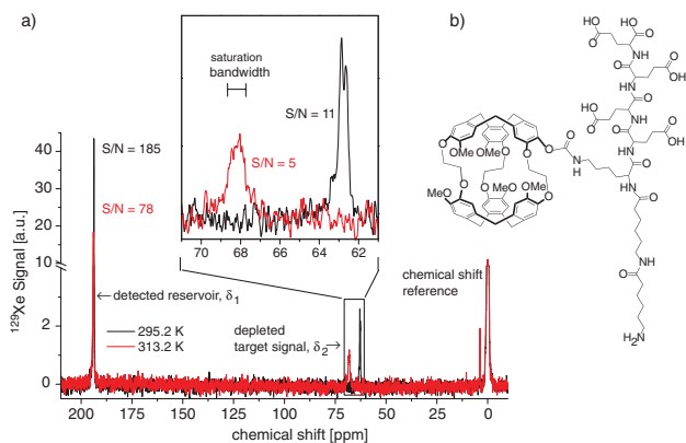
FIG. 1 (color). (a) ^{129}\text{Xe} NMR spectrum illustrating that only a small fraction of xenon is associated with a functionalized cryptophane cage at 33\ \mu\text{M} cage concentration. Increasing T from 295 K (black spectrum) to 313 K (red spectrum) shifts the signal of encapsulated xenon by ca. 5.5 ppm and induces accelerated chemical exchange that causes line broadening and decreases S/N . (b) Chemical structure of the functionalized cryptophane cage used in this study.
