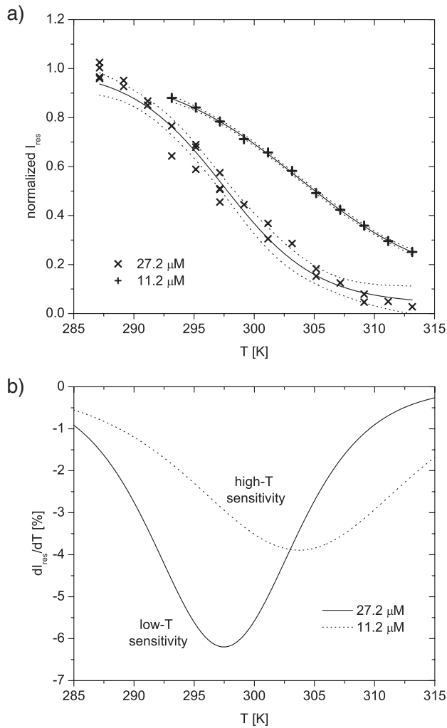
FIG. 3. (a) Calibration for temperature sensitivity of I_{\text{res}} shown in Fig. 2(b) at 27.2 \mu\text{M} cage concentration ( \times ) and for 11.2 \mu\text{M} cage concentration ( + ). The signal intensity is normalized to a control experiment without saturation pulse. Data are fitted to Eq. (1) and shown with a 95% confidence band (dashed lines). (b) The differential sensitivity of ^{129}\text{Xe} signal, intensity change per kelvin, is given by the first derivative of the fit results in (a). Reducing the concentration of the cage construct shifts the maximum sensitivity to higher temperatures. Since the experimental SD in determining I_{\text{res}} is \sim 3.6\% (see below), the temperature resolution is limited to ca. 0.6 K for the 27.2 \mu\text{M} solution.
