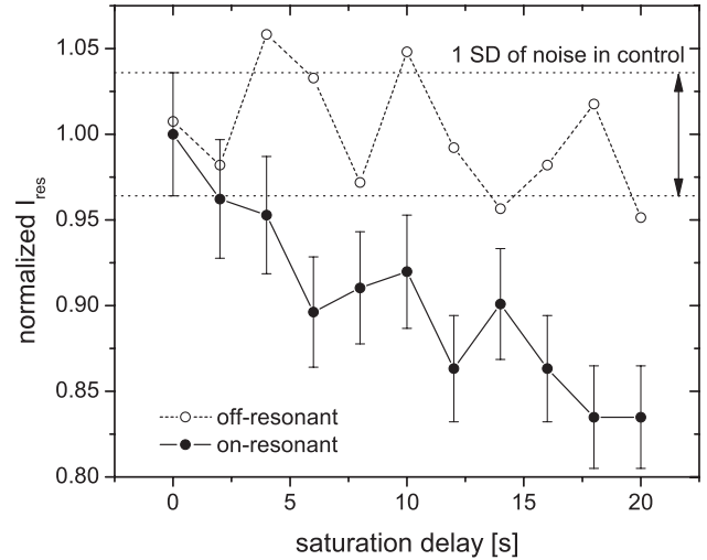
FIG. 4. High-sensitivity detection of 1.4 nM encapsulated xenon signal (10 nM cage present) in \text{D}_2\text{O} at 310 K. The SD in the control data set is 3.6% and is systematic noise due to imperfections in the xenon delivery. Maximum signal depletion is 16% of a resonance that was detected with a S/N of 110. However, the limiting factor for the hyper-CEST detection is the variability of 3.6% in the off-resonance experiment, so S/N for indirect sensor detection is 16.5/3.6 = 4.6 .
