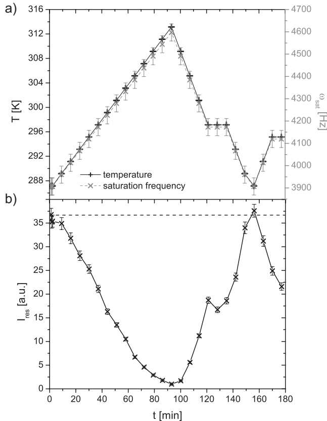
FIG. 2. (a) Input function T(t) (black solid line) for hyper-CEST signal transfer using the construct shown in Fig. 1. The saturation frequency offset \omega_{\text{sat}} (gray dashed line) is adjusted according to the resonance shift of 26.6 Hz/K. Bars indicate the bandwidth of the saturation pulse of \Omega = 76.7 Hz (0.925 ppm). (b) Response I_{\text{res}}(t) to T(t) . Varying the temperature changes ^{129}\text{Xe} signal transfer through the cage that is present at 27.2\ \mu\text{M} . The reference signal for no saturation transfer is illustrated by the dashed line.
