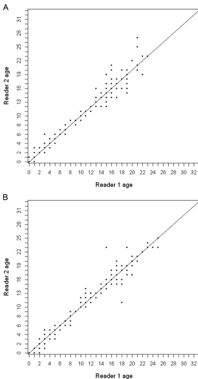
FIGURE 2. Age bias plots for readers 1 and 2 for the VIMS1983 (upper panel) and VIMS2004 (lower panel) data sets. In each panel the solid line has slope of 1 and an intercept of 0, representing no bias between readers.
