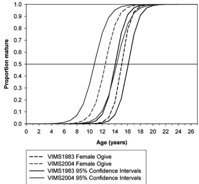
FIGURE 6. Ogives fitted to Sandbar Shark female maturity data for the VIMS1983 and VIMS2004 data sets using maximum likelihood estimation.
