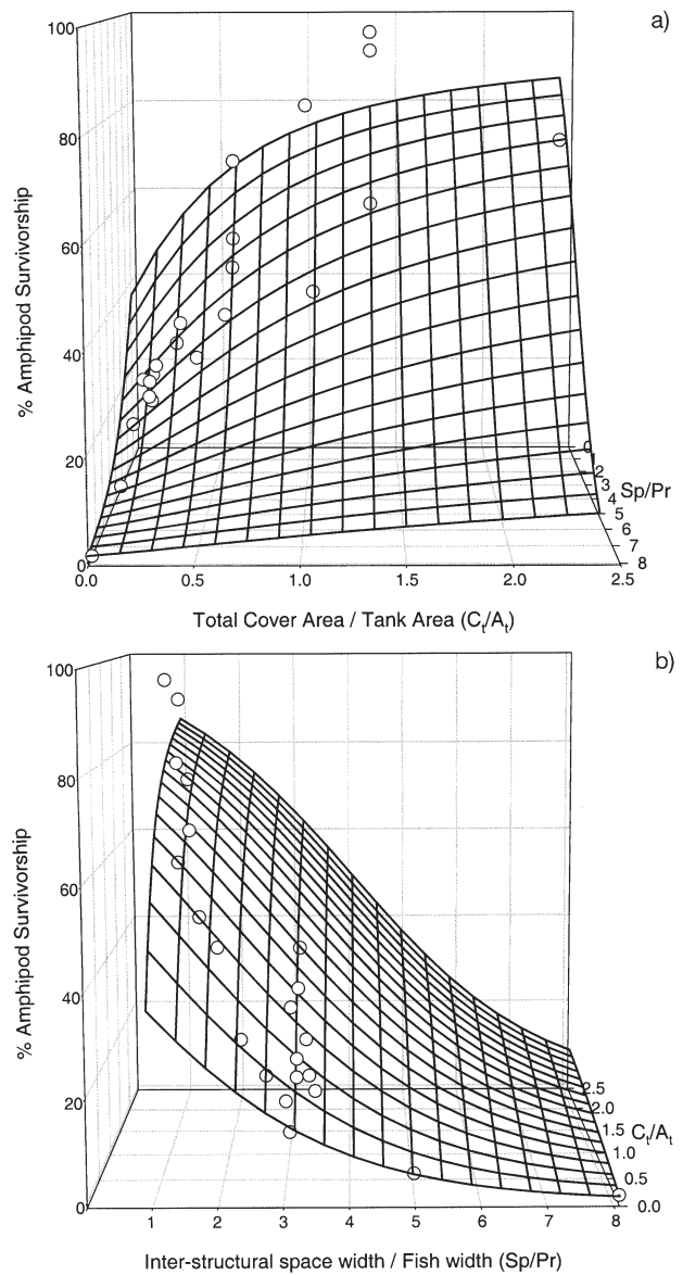
Fig. 3. (a) Three-dimensional plot of the results of the C_t/A_t experiment, combined with the results of the Bartholomew et al. (2000) lab experiments, and the modeled regression surface, viewed from the C_t/A_t axis. (b) The same, viewed from the Sp/Pr axis. See text for the regression surface equation
