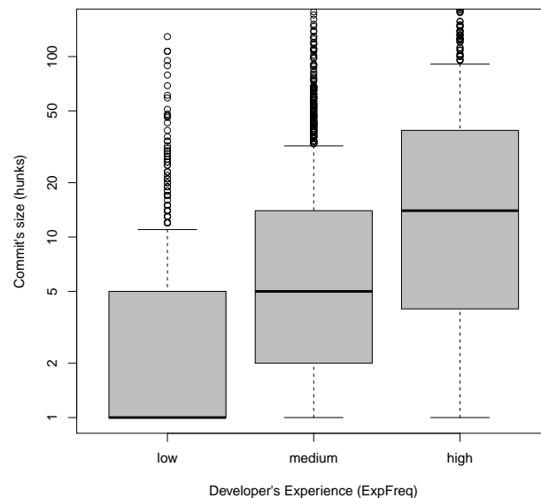
Figure 2. Boxplots of commit's size for developers having different levels of experience ( \log_4 j ). The boxplots, in log-scale, are produced using 768, 1,535 and 768 observations respectively for low, medium and high experience.
