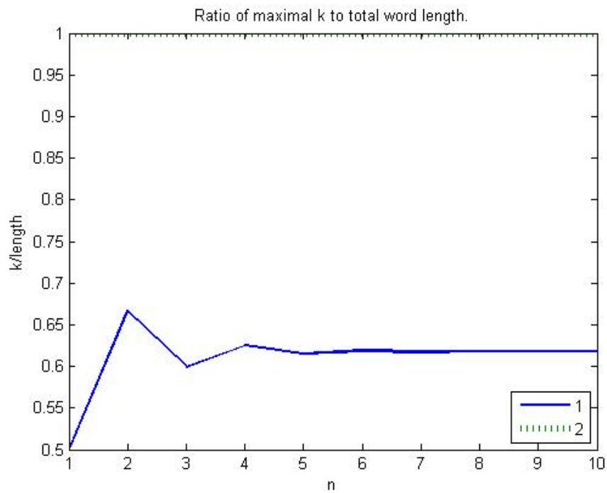
Figure 5.3: \max k / |\varphi^n(1)| and |\varphi^n(2)| versus n for the substitution \varphi(1) = 12 , \varphi(2) = 1 .
