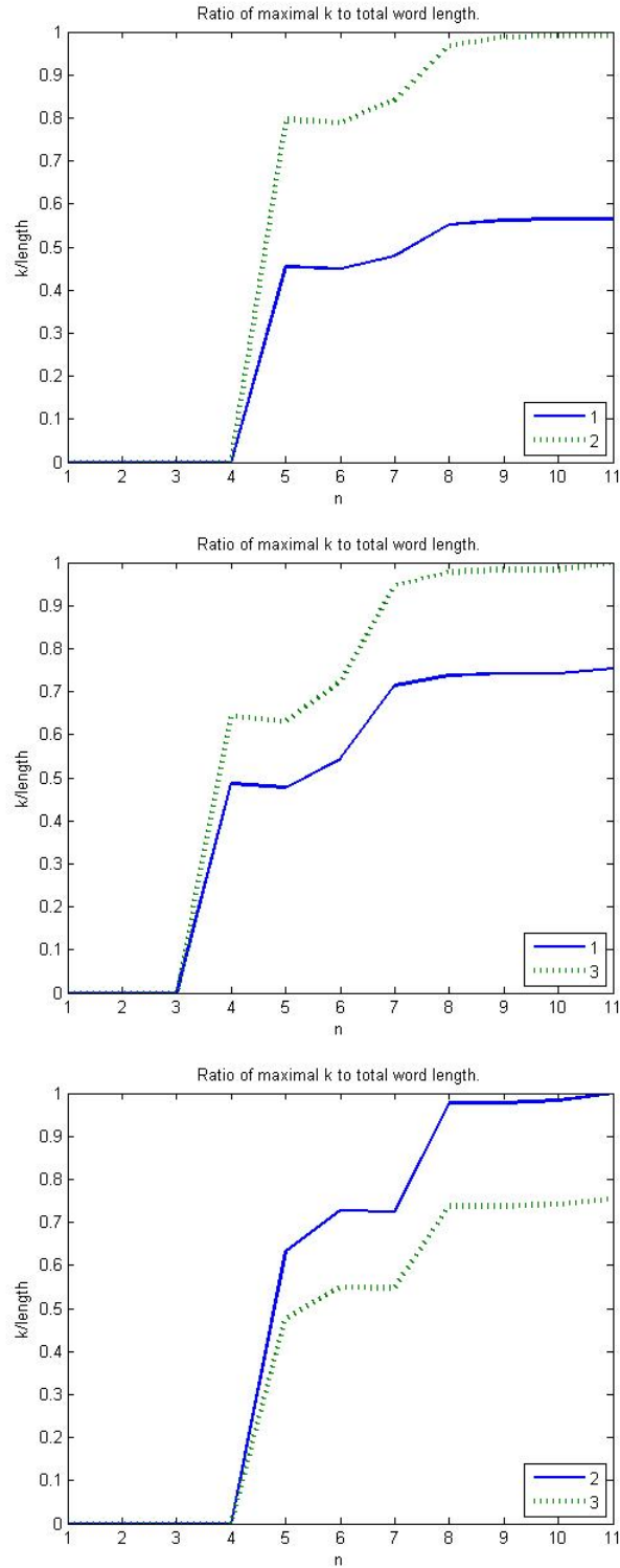
Figure 5.5: \max k / |\varphi^n(i)| and |\varphi^n(j)| versus n for the substitution \varphi(1) = 123 , \varphi(2) = 23 , \varphi(3) = 31 .
