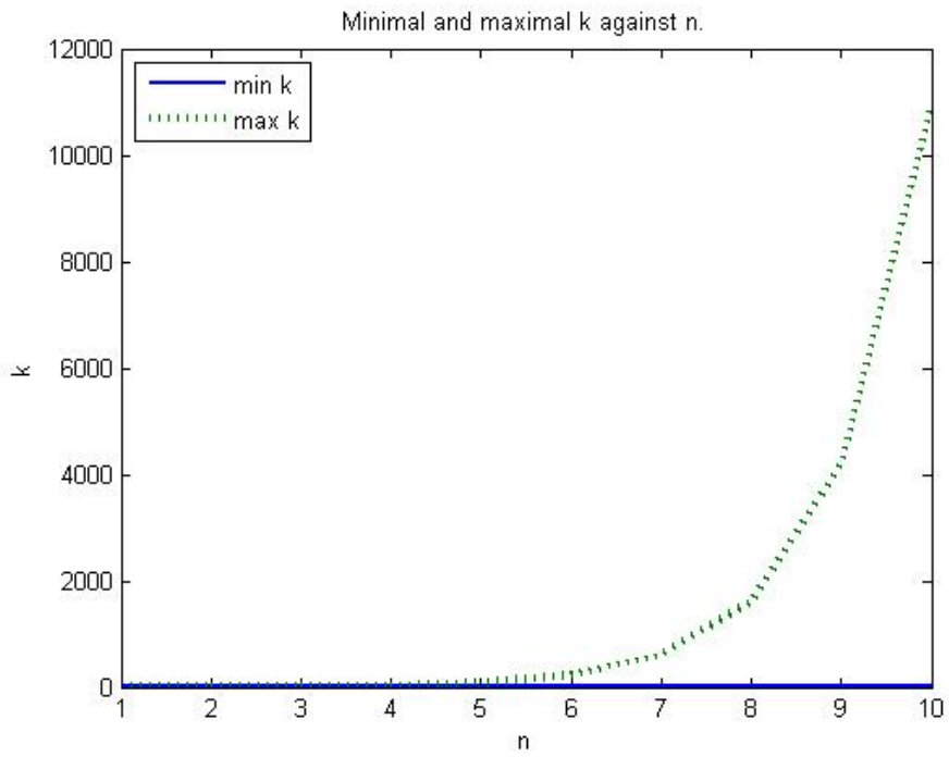
Figure 5.2: \min k and \max k versus n for the substitution \varphi(1) = 122 , \varphi(2) = 21 .
