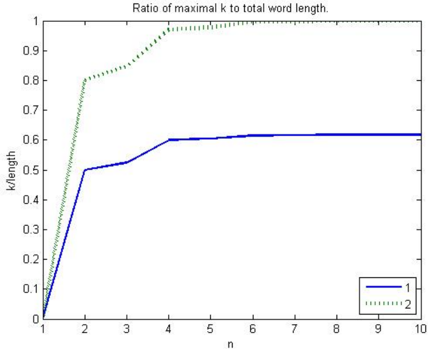
Figure 5.4: \max k / |\varphi^n(1)| and |\varphi^n(2)| versus n for the substitution \varphi(1) = 112 , \varphi(2) = 21 .
