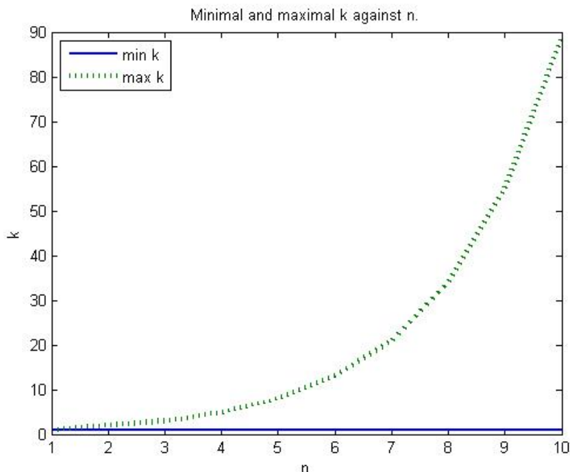
Figure 5.1: \min k and \max k versus n for the substitution \varphi(1) = 12 , \varphi(2) = 1 .
