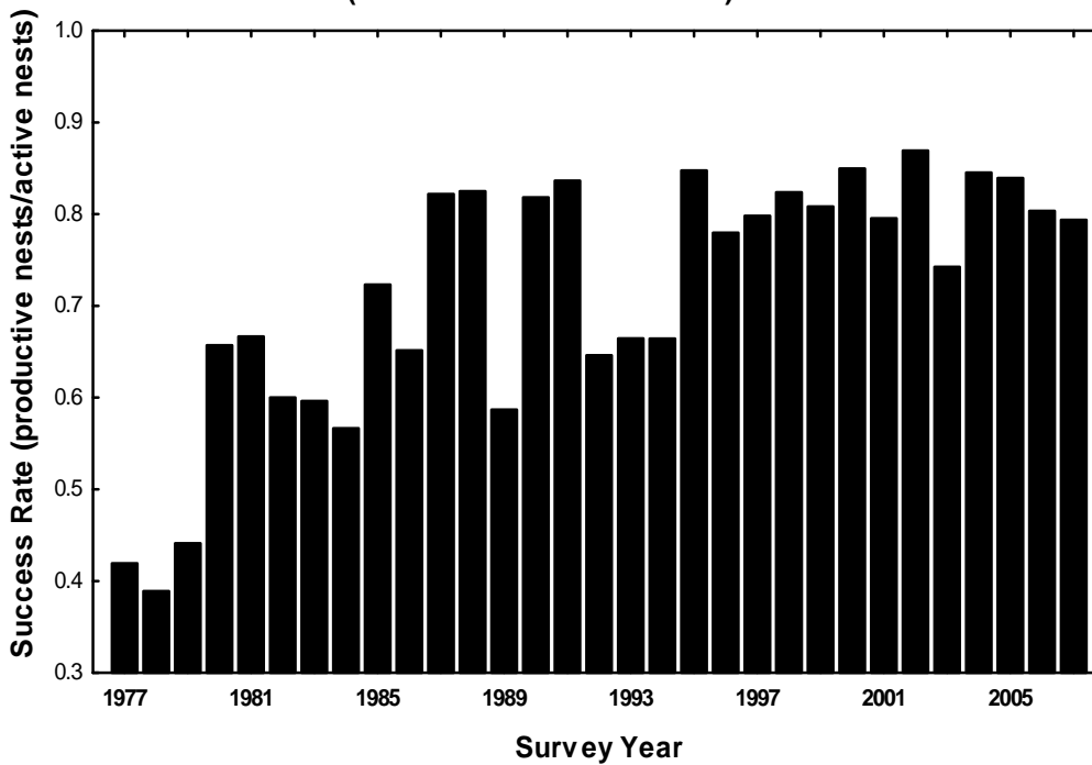
Figure 4. General trend in success rate for Bald Eagles in Virginia (1977-2007)
