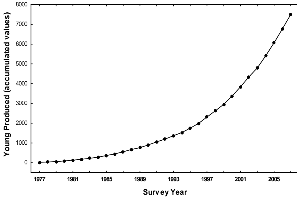
Figure 3. Productivity accumulation curve for Bald Eagles in Virginia (1977-2007). Total chicks produced over the 31-year study was 7,505.
