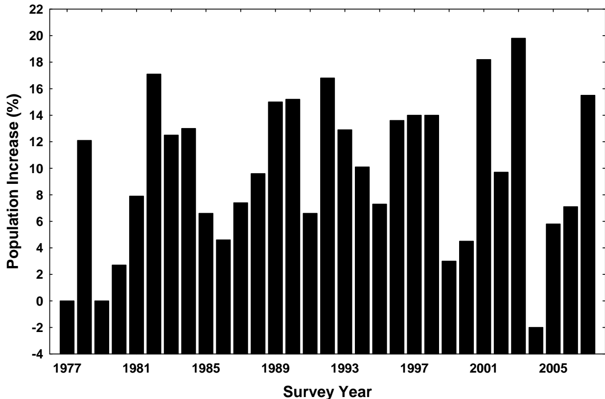
Figure 1. Annual increase values for the 31-year survey period (1977-2007). Values calculated as (\text{Pairs}_t - \text{Pairs}_{t-1}) / \text{Pairs}_{t-1} \times 100 .
