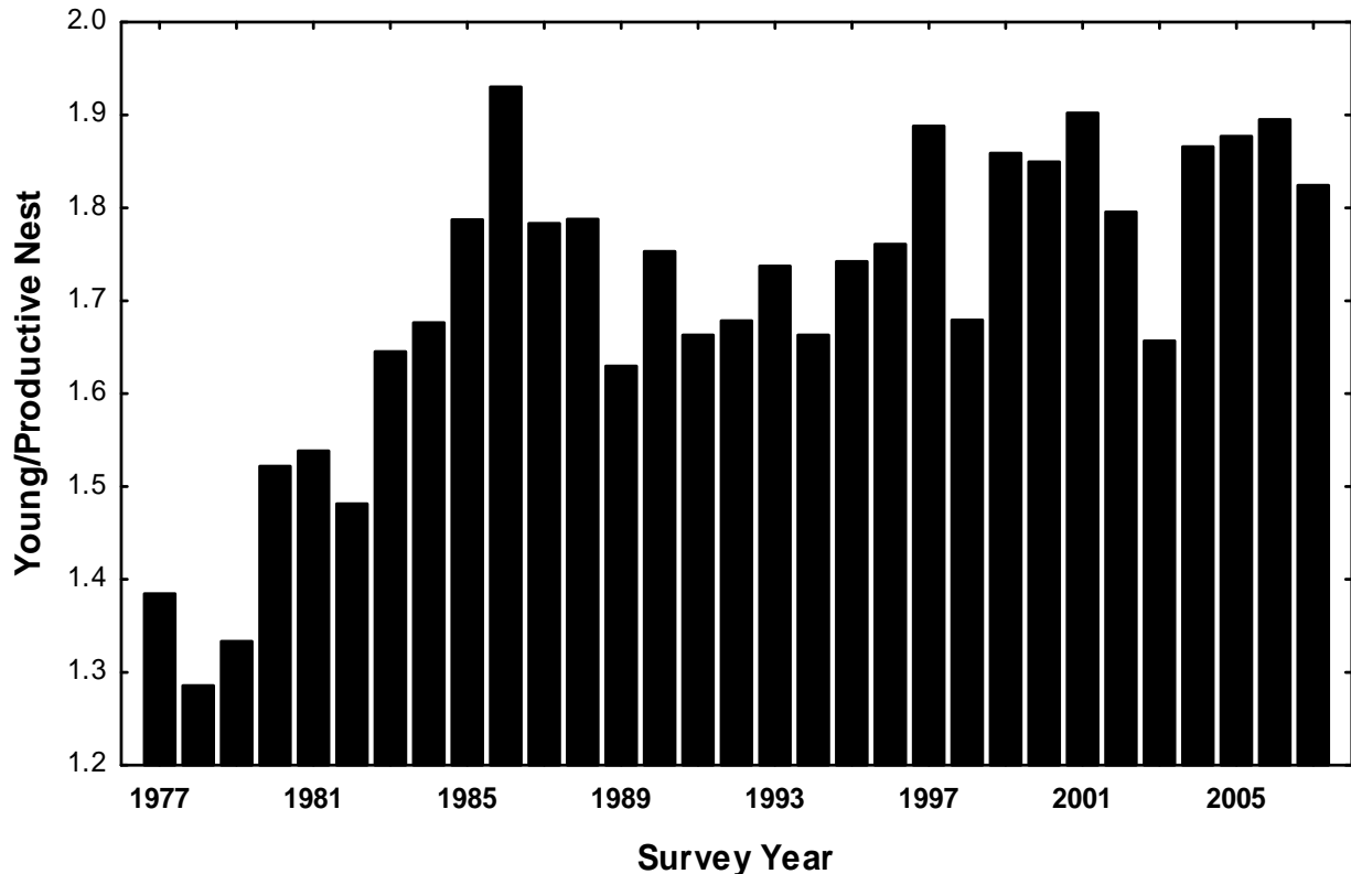
Figure 5. Temporal trend in average brood size for Bald Eagles in Virginia (1977-2007).
