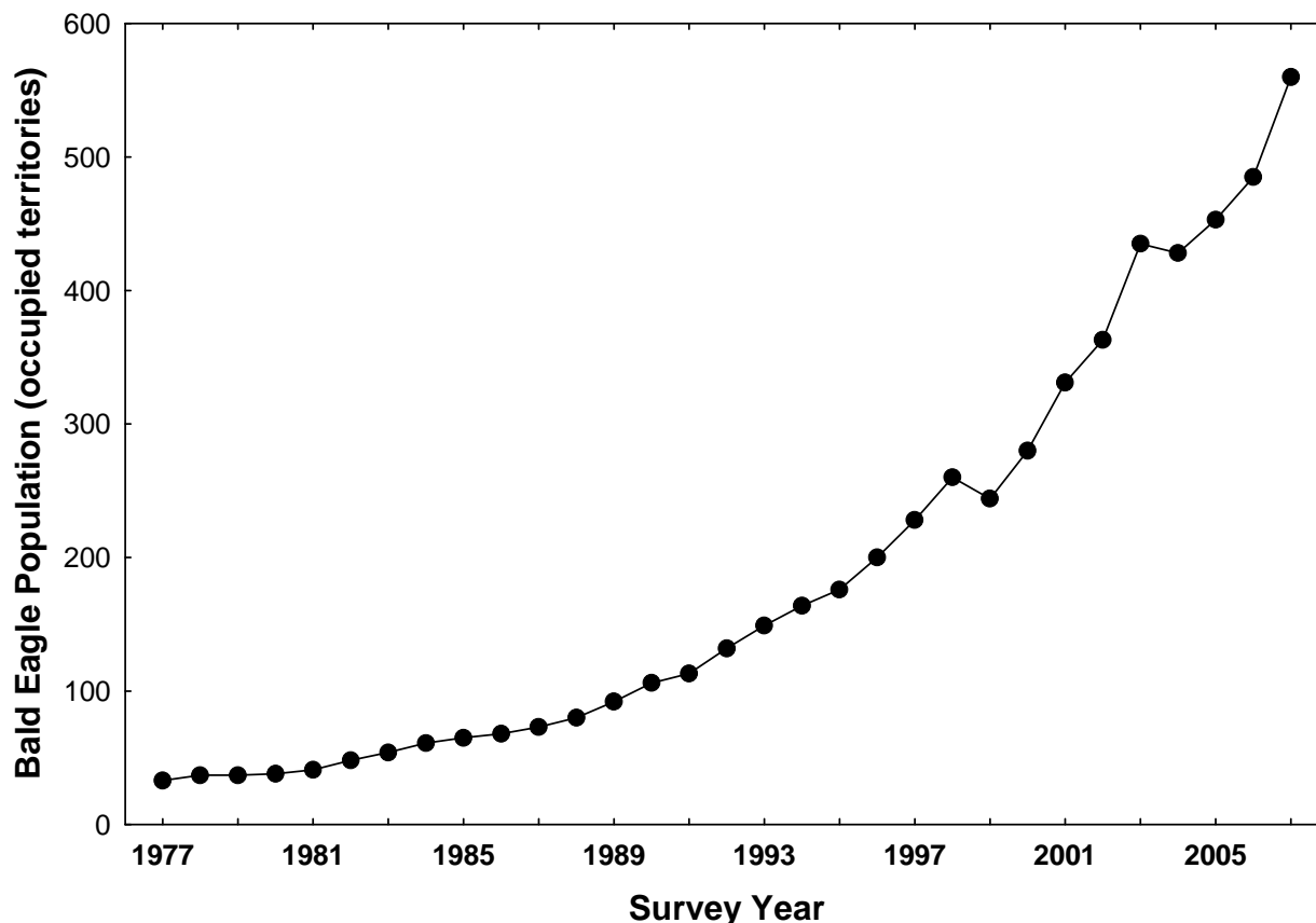
Figure 2. Change in the Virginia Bald Eagle breeding population 1977-2007.
