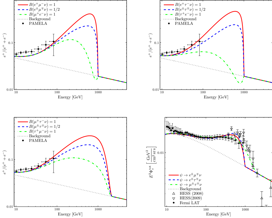
Figure 4.3: Positron fraction and total electron-positron flux for some charged-lepton-flavor-violating decays with various sets of branching fractions. Best fits are shown, corresponding to the following masses and lifetimes: for \psi \rightarrow e^\pm \mu^\mp \nu , m_\psi = 2.0 TeV and \tau_\psi = 2.9 \times 10^{26} s; for \psi \rightarrow e^\pm \tau^\mp \nu , m_\psi = 2.0 TeV and \tau_\psi = 2.4 \times 10^{26} s; for \psi \rightarrow \mu^\pm \tau^\mp \nu , m_\psi = 4.5 TeV and \tau_\psi = 1.0 \times 10^{26} s.
