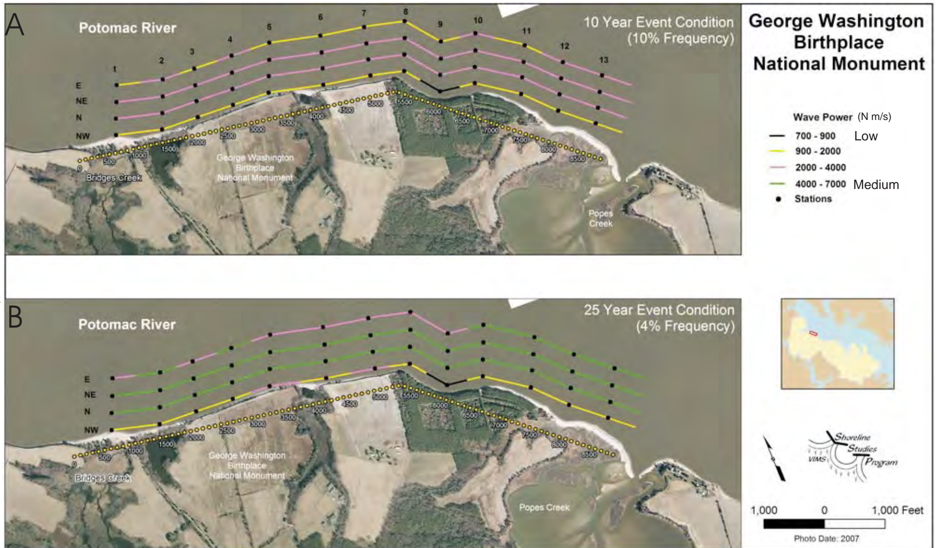
Figure 29. Wave power at 13 alongshore stations for the A) 10 year and B) 25 year storm condition with different directions.
