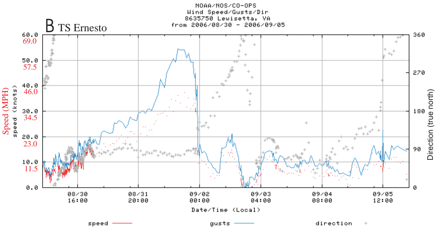
Figure 8. Wind speeds and directions at Lewisetta during A) Hurricane Isabel and B) Tropical Storm Ernesto.
