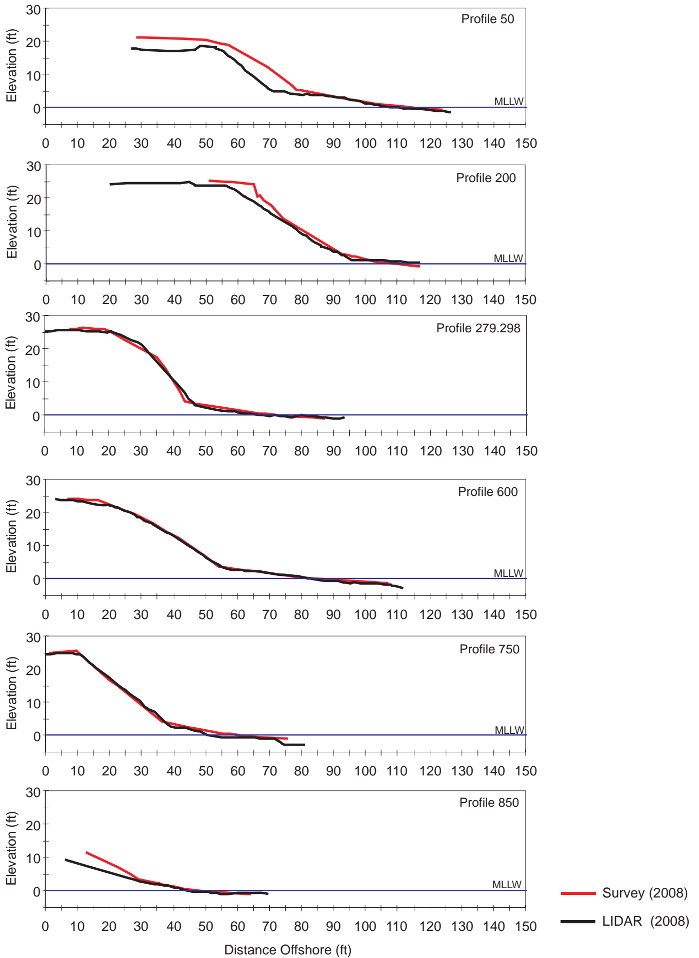
Figure 27. Comparison between ground survey and LIDAR at selected profiles along Popes Creek (locations as shown on Figure 5).
