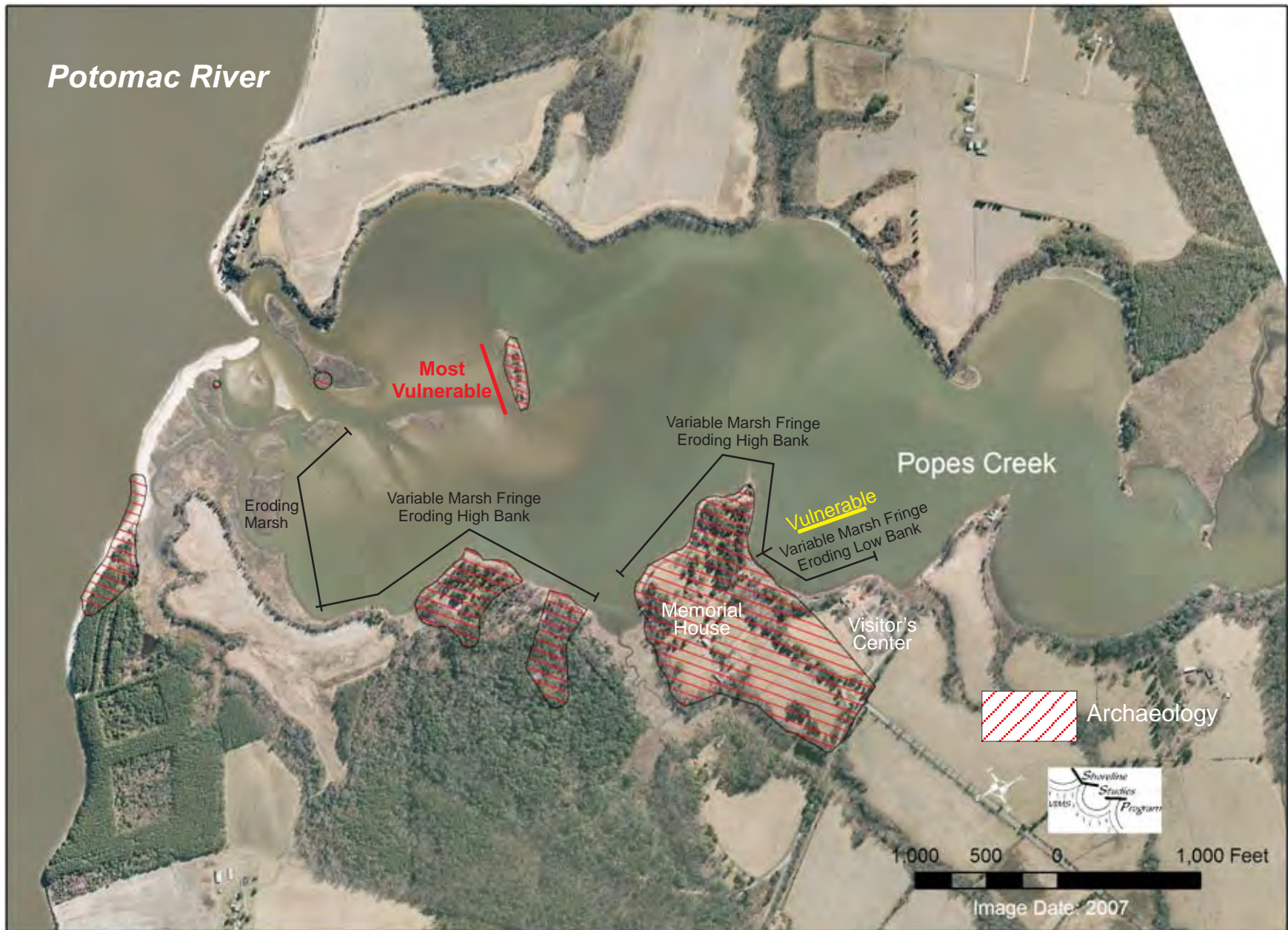
Figure 32. Summary of major findings and vulnerability map for GEWA's Popes Creek shoreline.
