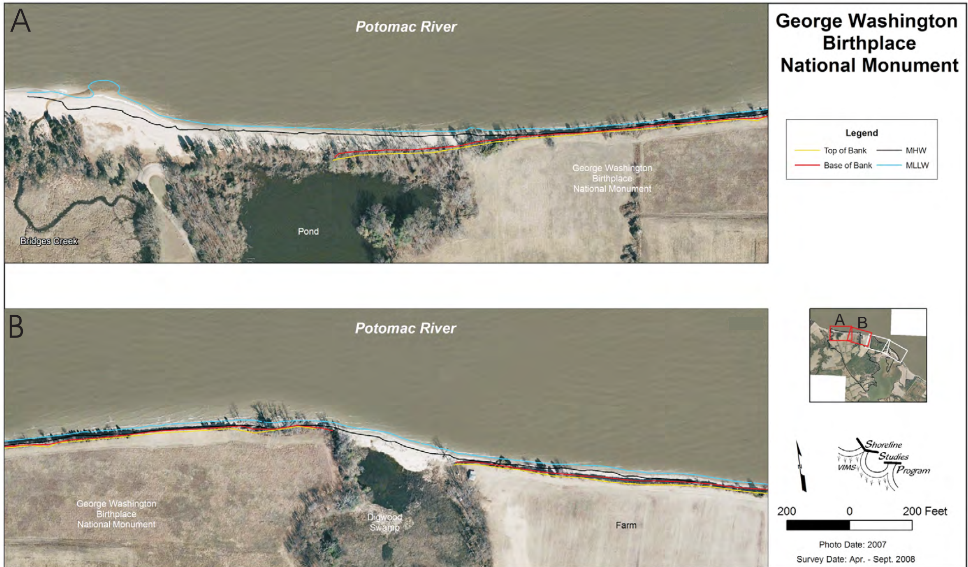
Figure 22. RTK-GPS survey results showing the top of bank, base of bank, mean high water, and mean lower low water along GEWA's western Potomac River shoreline.
