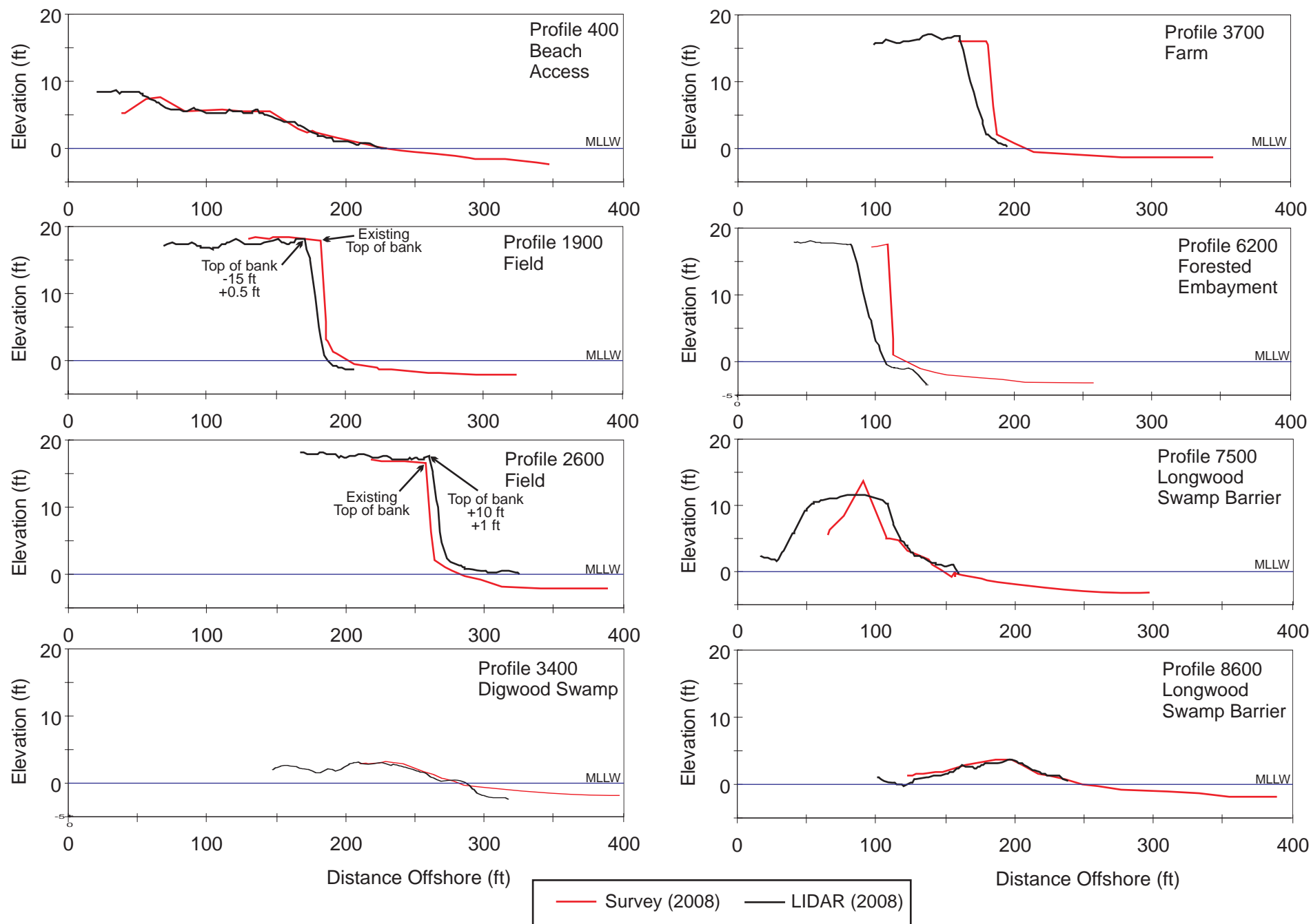
Figure 26. Comparison between ground survey and LIDAR at selected profiles along GEWA's Potomac River shoreline (locations as shown on Figure 4).
