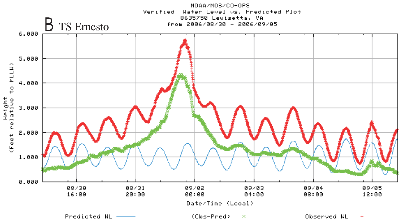
Figure 9. Tide gauge data at Lewisetta, Virginia during A) Hurricane Isabel and B) Tropical Storm Ernesto. The red line shows the measured water level in feet relative to MLLW; the blue line represents the predicted tide; the green line shows the difference between the observed and predicted water levels and is commonly referred to as the storm surge.
