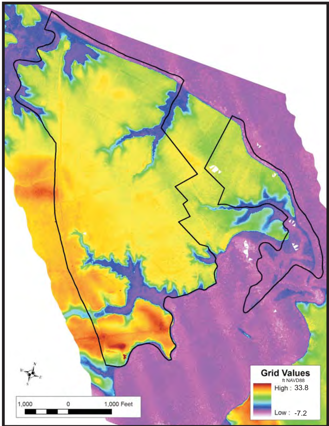
Figure 6. Digital Elevation Model of the 2008 LIDAR data.
