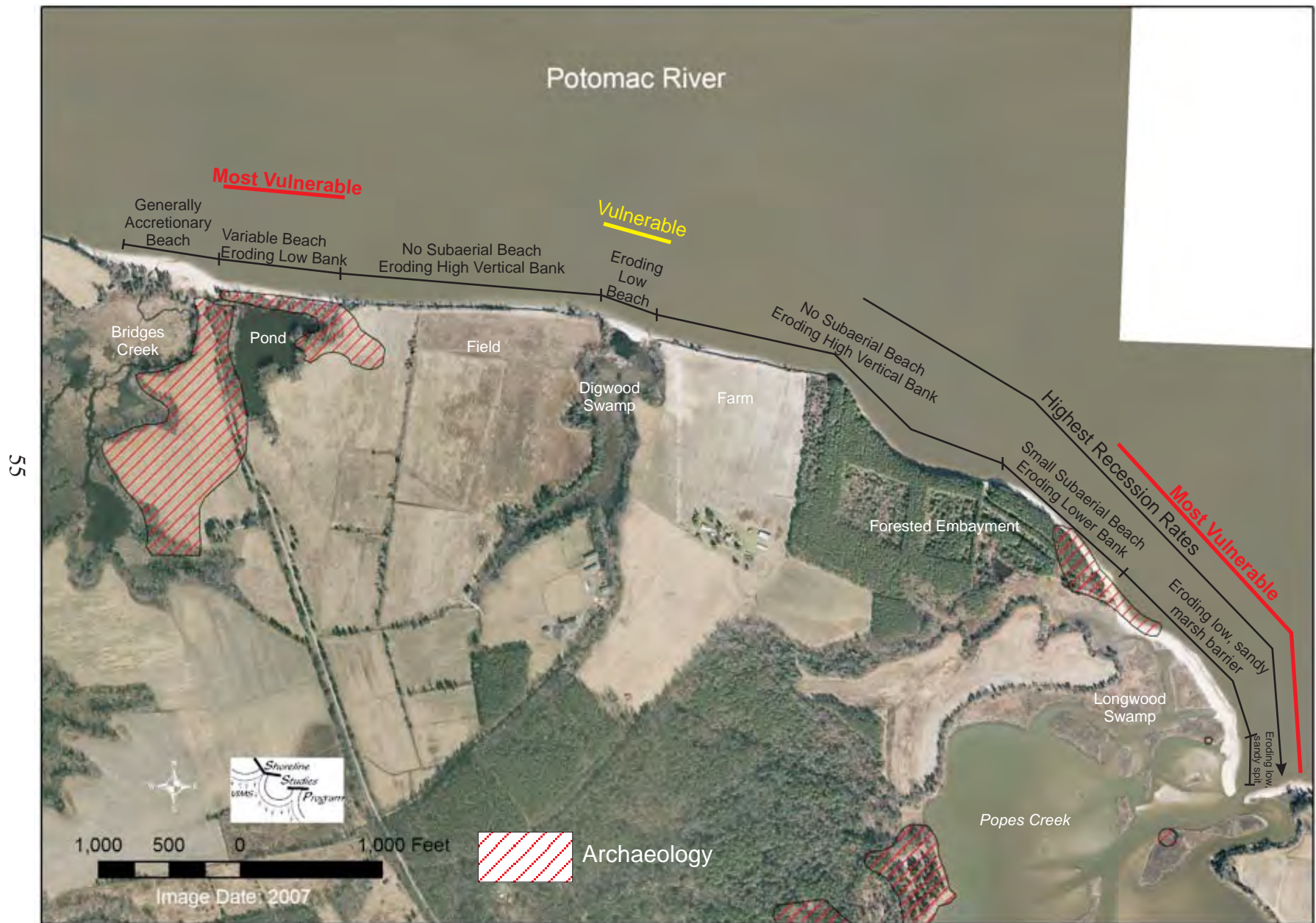
Figure 31. Summary of major findings and vulnerability map for GEWA's Potomac River shoreline.
