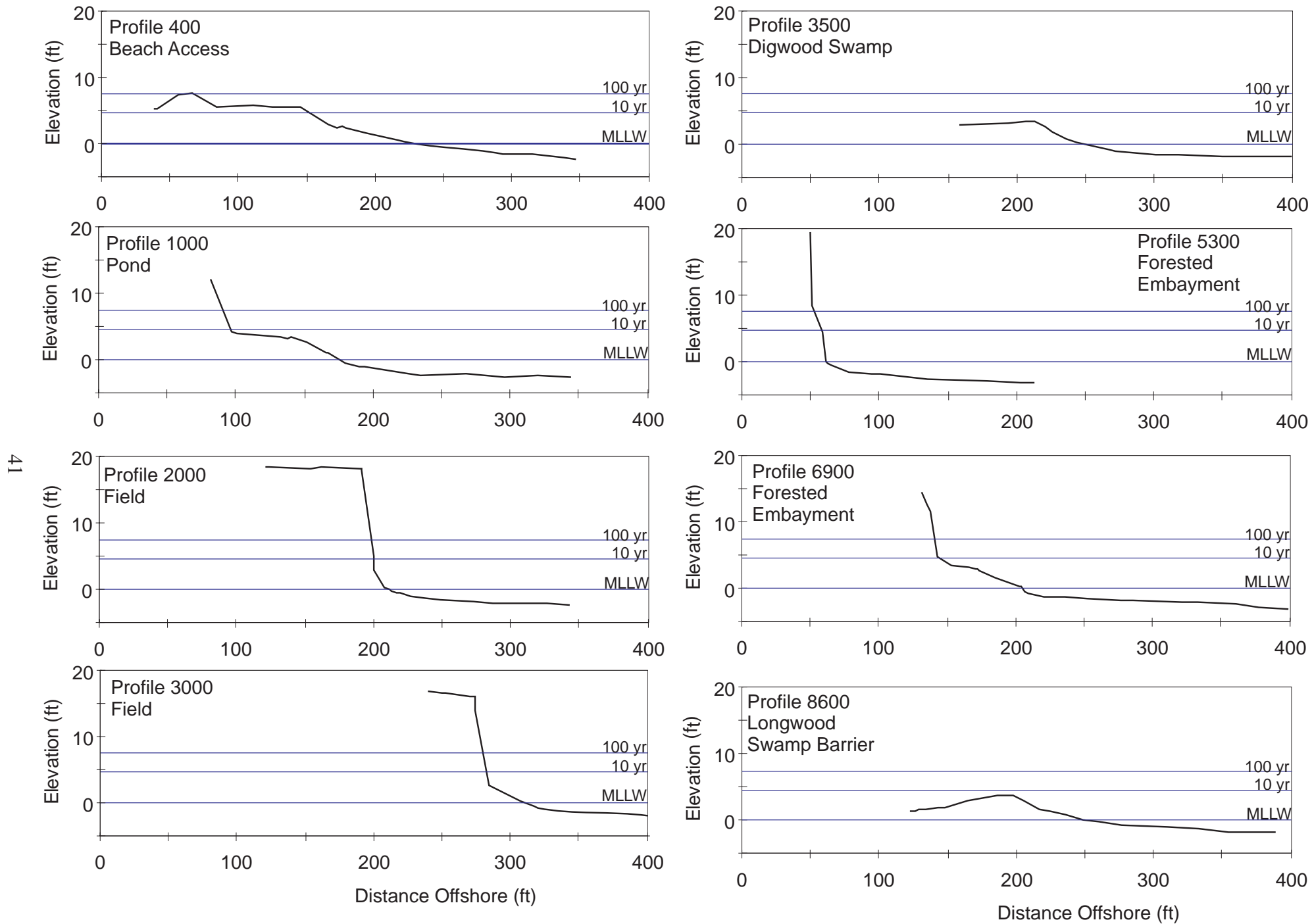
Figure 24. Typical profiles of different sections of GEWA's Potomac River Shoreline. Reference Figure 4 for profile locations.
