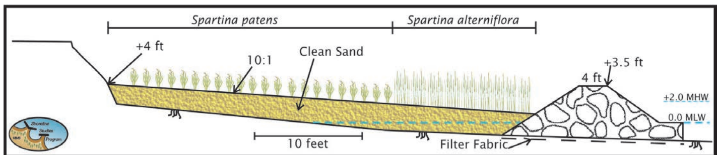
Appendix 3, Figure 1. Typical cross-section for a low sill that is appropriate for low to medium energy shorelines of Fairfax County. The project utilizes clean sand on an 10:1 (H:V) slope, and the bank can be graded to a (minimum) 2:1 slope, if appropriate.
