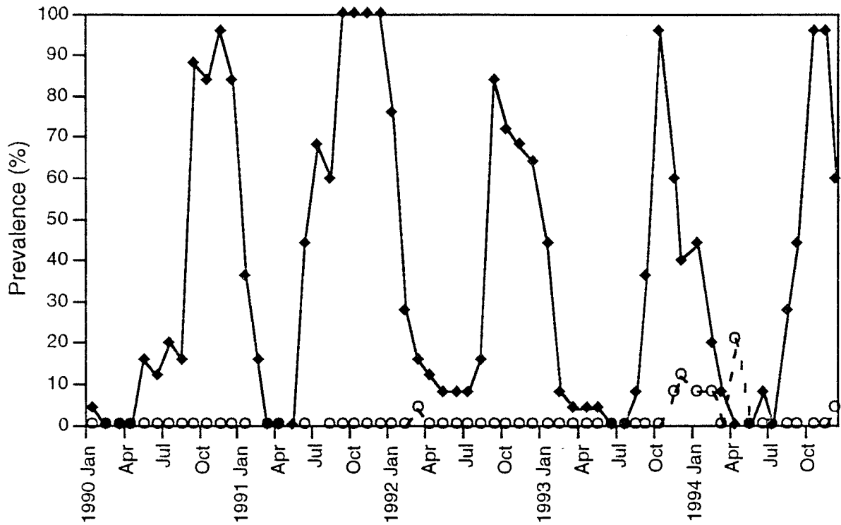
Figure 6. Salinity (top) and prevalence (bottom) of P. marinus (solid line) and H. nelsoni (dashed line) at Horsehead Rock, VA for the years 1990-1994.
