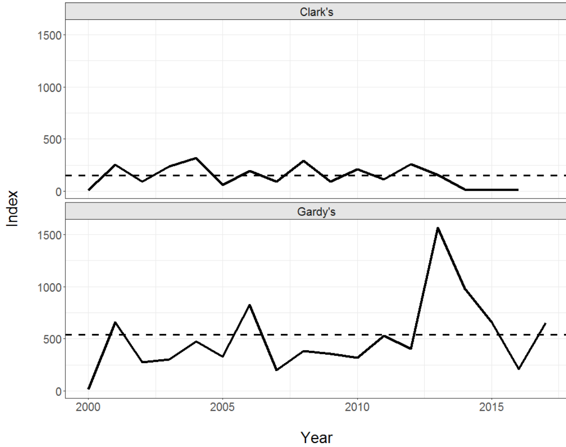
Figure 4. Elver eel index (area-under-the-curve method) from 2000 to 2017. Collections in 2000 followed different protocols and are not directly comparable to collections in later years. Time-series averages consist of data from 2001 to 2017. Sampling at Clark's Millpond was discontinued after 2016.
