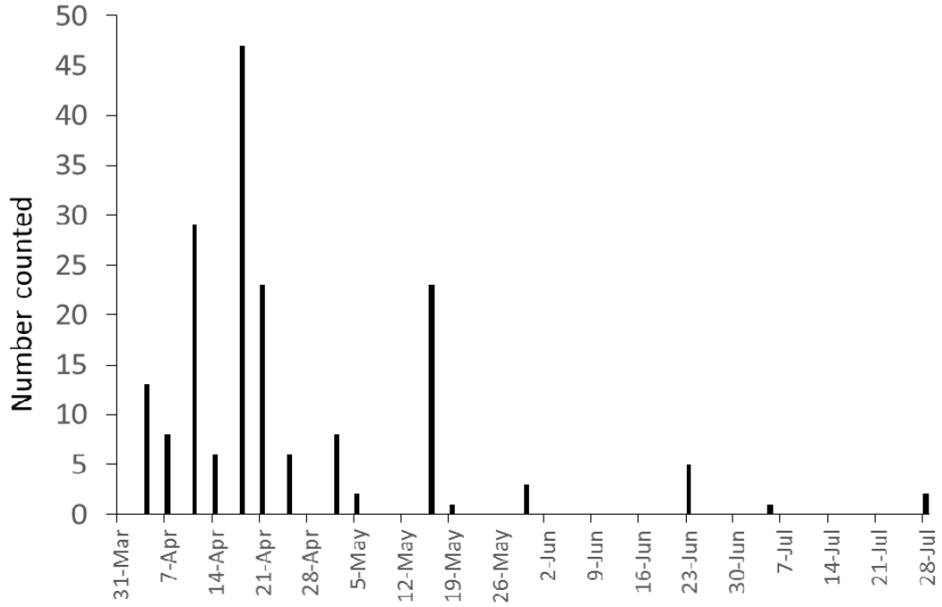
Figure 8. Number of fully pigmented glass eels captured at Gardy’s Millpond from 31 March to 28 July, 2017; N = 184 eels. We combined these fully pigmented glass eels with elvers in this report to remain consistent with previous reports.
