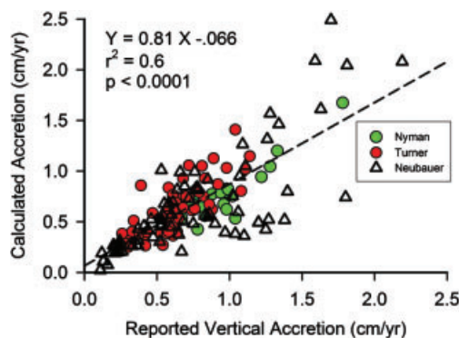
Figure 2. Mixing model-calculated accretion rates and reported ^{137}\text{Cs} -based vertical accretion rates. Calculations used published mass accretion rates ( \text{g m}^{-2} \text{yr}^{-1} ) of inorganic and organic matter as reported in Nyman et al. [1993, 2006], Turner et al. [2000], and Neubauer [2008].
