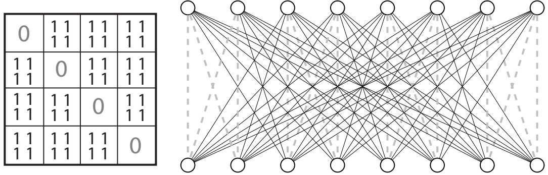
Figure 1.2: Left: L_{8,2} . Right: G(L_{8,2}) .
