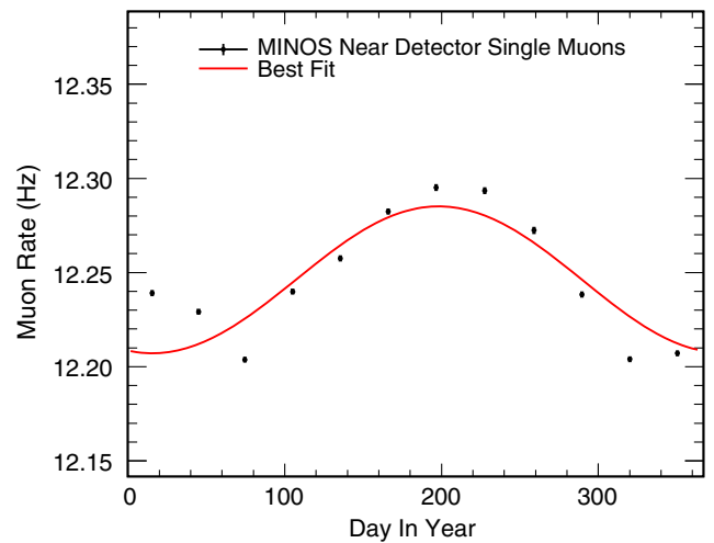
FIG. 7 (color online). The top figure is the multiple-muon rate in the ND, binned according to calendar month, which each point showing the average rate for all years of data taking. The figure also shows a cosine fit to the data. The single-muon rate is shown in the bottom figure, showing a clearly different seasonal modulation.
