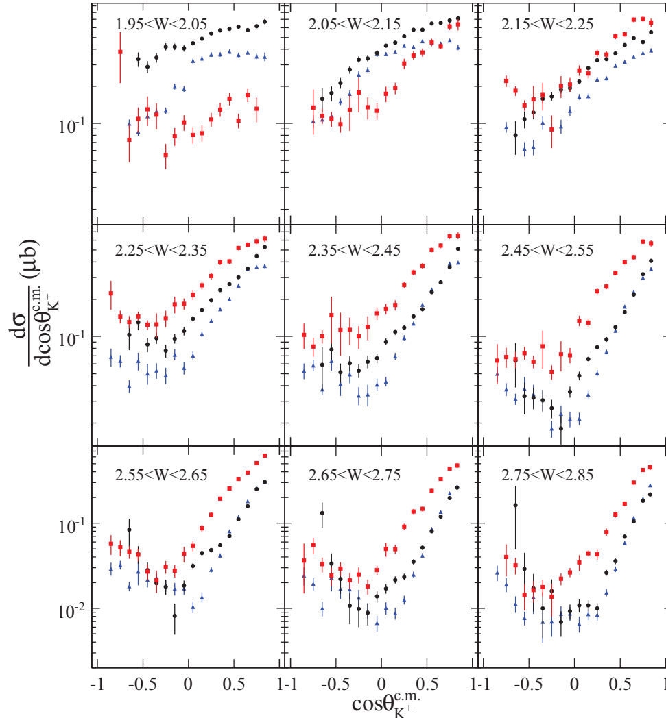
FIG. 17. (Color online) Comparison of differential cross sections of the \Sigma^0(1385) (black circles), \Lambda(1405) (blue triangles), and \Lambda(1520) (red squares) as a function of kaon production angle \cos\theta_{K^+}^{\text{c.m.}} for each 100 MeV wide bin in energy W (GeV). For the \Lambda(1520) the threshold bin has 2.02 \leq W \leq 2.05 GeV.
