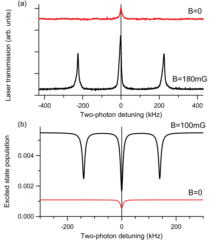
FIG. 3. (Color online) (a) Examples of measured CPT resonances at B = 0 and B = 180 mG. Laser intensity before the cell is 8.4 \text{ mW/cm}^2 . (b) Calculated excited-state population \pi_e versus two-photon detuning at B = 0 and B = 100 mG. Total resonant intensity I_1 + I_2 = 10 \text{ mW/cm}^2 .
