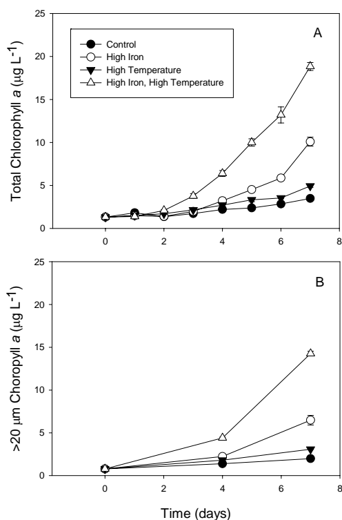
Fig. 1. Size-fractionated chlorophyll- a concentrations. (A) 0.2 \mu\text{m} , total phytoplankton assemblage; (B) >20 \mu\text{m} size fraction. Error bars indicate one standard deviation.
