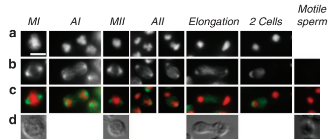
Figure 4 | Microtubule dynamics during and following the meiotic divisions. (a–c) In methanol fixed sperm spreads, DNA was labelled with DAPI (a) and tubulin was labelled with FITC-conjugated anti- \alpha -tubulin monoclonal DM14 (Sigma) (b). In the merge image (c), DNA is red and tubulin is green. Spindles are symmetric during metaphase I and II, but become biased towards the X-chromosome side during anaphase II. During the elongation stage, microtubules reposition to the spermatid that has the smaller chromatin mass. (d) DIC images. All images are at the same scale; scale bar, 3 \mu m. MI , metaphase I; AI , anaphase I; MII , metaphase II; AII , anaphase II.
