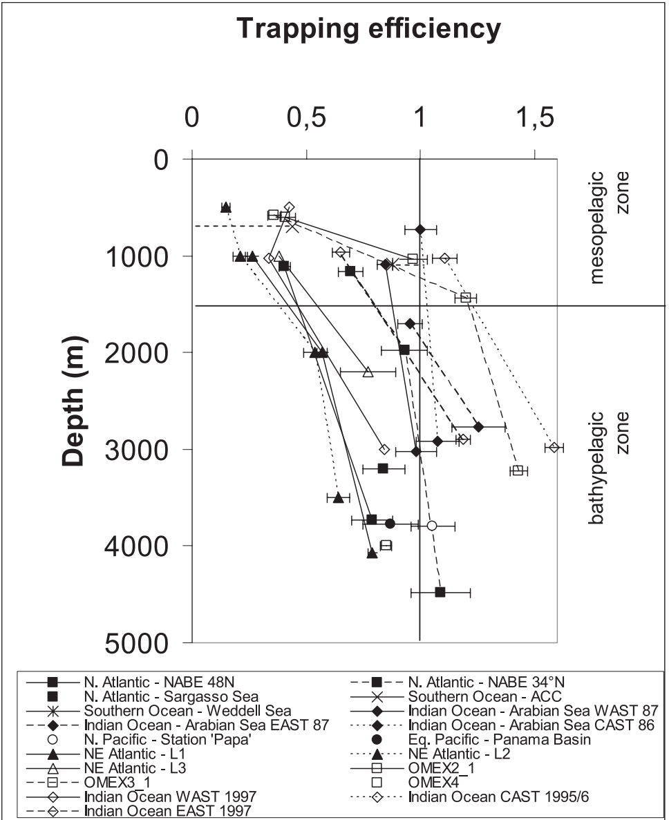
Figure 5.5. Trap collection efficiencies derived from 230 Th and 231 Pa measurements in sediment trap and water column samples according to Bacon (1988). Data from Yu et al. (2001); Scholten et al. (2001, 2005). Arabian Sea data are from deployments generally shorter than one year but they include the monsoon period and may be overestimated. OMEX deployments are near the continental margin where deeper traps may be influenced by lateral advection.
