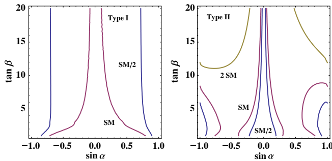
FIG. 3 (color online). For the type I and type II models discussed in the text, we plot the ratio \frac{N_{2HDM}}{N_{SM}} in the (\tan\beta, \sin\alpha) plane for h \rightarrow \bar{b}b . The results for the lepton-specific (flipped) model are very similar to those for the type I (type II) model. Along the red (SM) lines, the ratio is 1.0, along the blue (SM/2) lines it is 0.5, and along the gold (2SM) lines it is 2.0. In the type I case, the ratio is less than 1.0 for virtually all of the parameter space.
