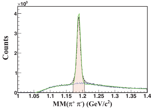
FIG. 4. (Color online) Reconstructed \Sigma^+ signal (dashed line) in the missing mass of the two charged pions, with the \pi^0 and the K_S^0 selected, and with the collinearity angle cut as described in the text. The dotted line is the MM(\pi^+\pi^-) distribution from the sidebands of the K_S^0 with a \pi^0 selected and with the same collinearity angle cut as above. No normalization or scaling is done. The fit (solid line) includes a Gaussian for the peak and a second order polynomial for the background. The shaded region shows the \pm 3\sigma cut around the peak to select the \Sigma^+ .
