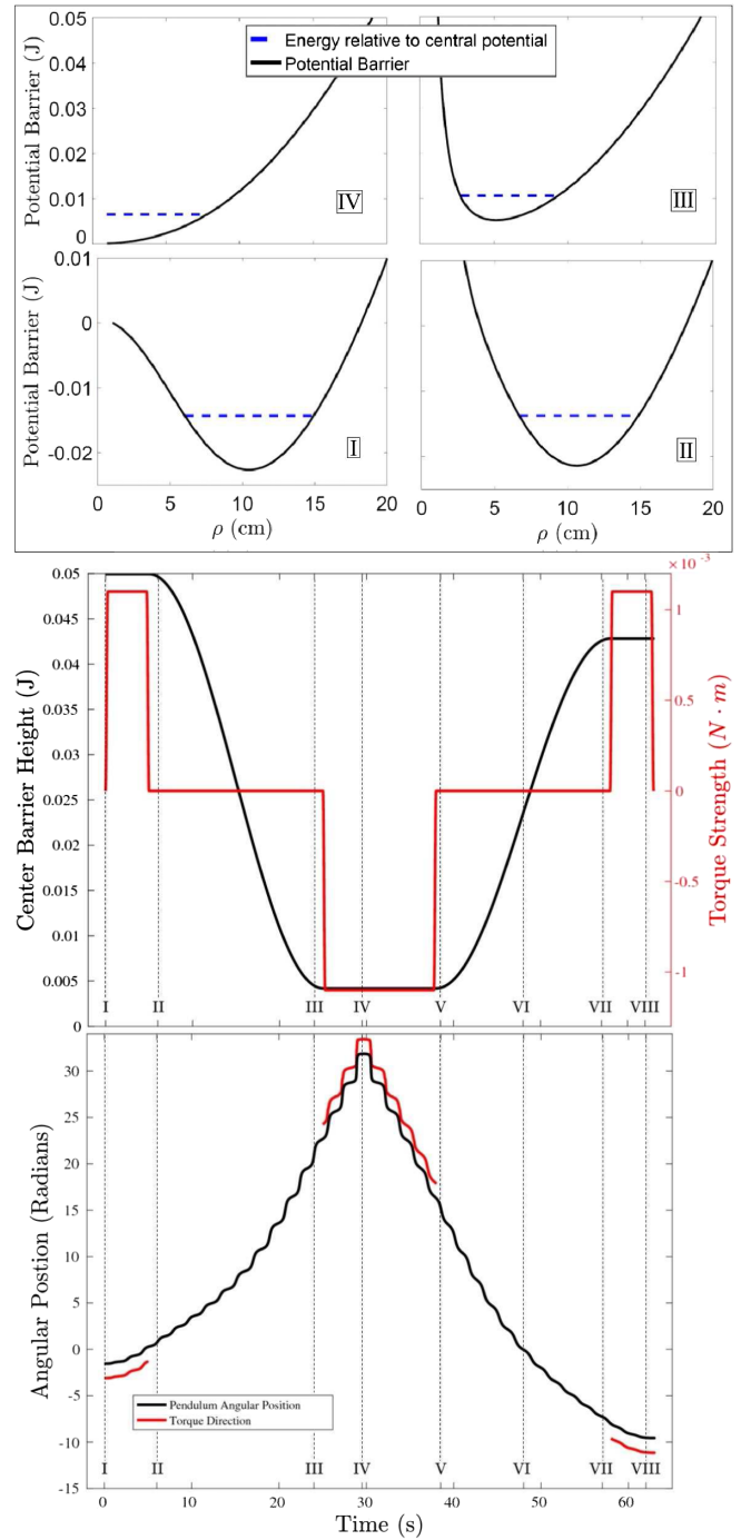
FIG. 4. Top: our potential, V(\rho) + \ell^2/(2m\rho^2) , at the first four time steps. Zero energy is in reference to the coil potential energy at \rho = 0 . Middle: timing sequence of our experiment, showing the barrier height and magnitude of torques on each particle. The difference in initial and final barrier heights is a characterization of the energy lost due to friction over the course of the experiment. Bottom: representative timing sequence of the torque coils tailored a priori to keep an azimuthal applied force for a particular trajectory (this figure is shown for the particle that begins on the outer turning radius).
