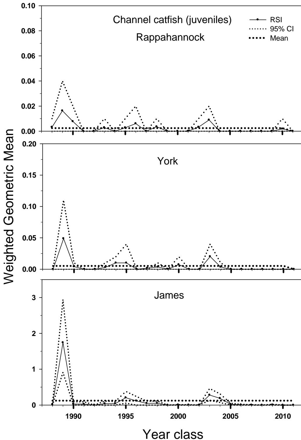
Figure 11. Juvenile channel catfish random stratified indices ( RSI_{GM} , 95% C.I.) and time series averages (dotted line) based on the RSI_{GM} 's from the Rappahannock, York, and the James rivers. Note change in scale on y-axes.
