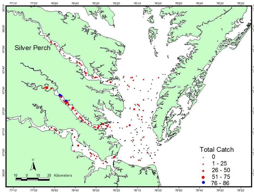
Figure 16. Juvenile Silver Perch random stratified ( RSI_{GM} , 95% C.I.), fixed transect (Rivers only – RO), and Bay and fixed river station (BRI) indices and the time series average (dotted line) based on the RSI_{GM} (Top), and distribution of juvenile Silver Perch from index strata and months (Bottom).
