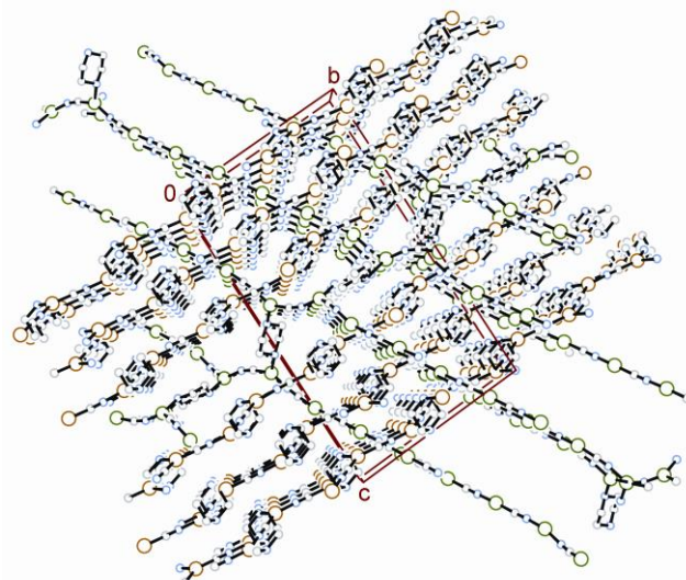
Fig. 1 Packing diagram of 1 showing interpenetrating sub-lattices. Cu atoms large circles, orange = sublattice A atoms and green = sublattice B atoms, N and C atoms small blue and grey circles, H atoms omitted for clarity. Distances for Cu–X (X = disordered C/N) = 1.843(5)–1.900(4) Å, distances for Cu–N(Pip) = 2.049(7)–2.144(4), distances for X=X = 1.128(8)–1.168(6) Å, angles Cu–X=X = 160.9(6)–178.8(4)°, and angles for X–Cu–X = 134.5(3)–143.6(2)° for 3-coordinate Cu atoms and 165.2(3)–179.76(19)° for 2-coordinate Cu atoms.
