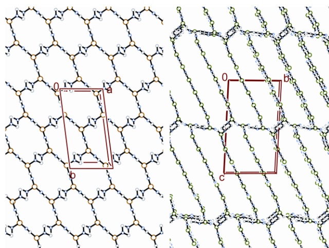
Fig. 2 Isolated views of 1 sub-lattices. Left: Sub-lattice A, right sub-lattice B. Cu atoms large orange and green circles, N and C atoms small blue and grey circles, H atoms omitted for clarity.
