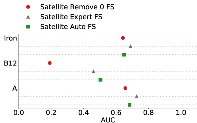
FIGURE 3 Comparison feature selection methods, including removing any features without data, human expert feature selection, and our K-medoids method, all in region WCO. WCO, West Coast.
