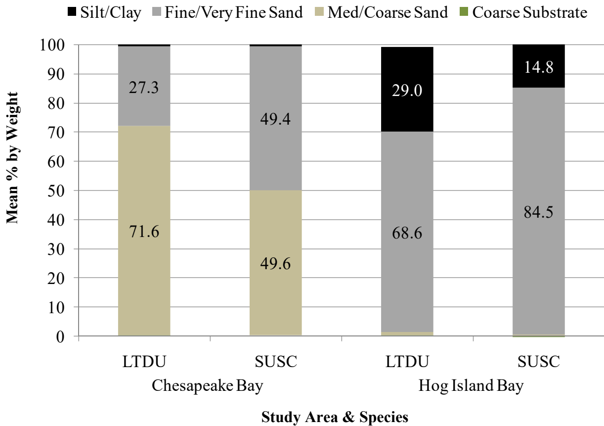
Figure 12. Mean % grain size for sediment collected from sea duck foraging areas in both study areas for both duck species (see Methods section for size class definitions).
