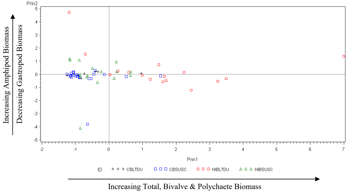
Figures 17. Principle Components Analysis output for biotic factors of benthic samples.
