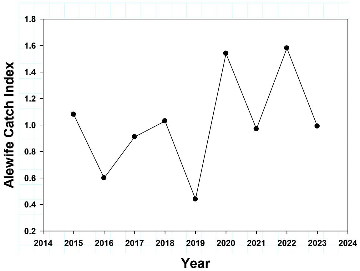
Figure 12. Recent (2015-2023) values of the catch index of female Alewife on the Chickahominy River.
