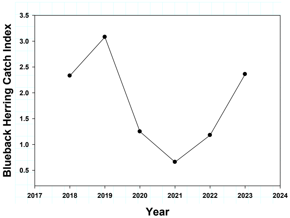
Figure 15. Recent (2018-2023) values of the catch index of female Blueback Herring on the Rappahannock River.
