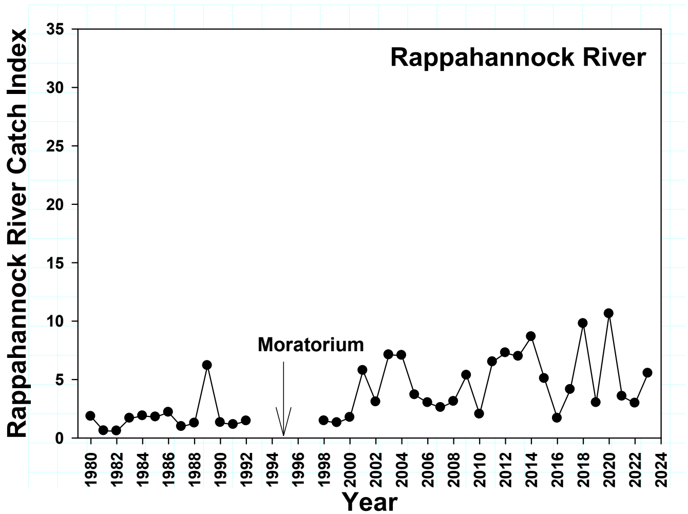
Figure 10. Recent (1998-2023) and historic values of the catch index of female American shad on the Rappahannock River.
