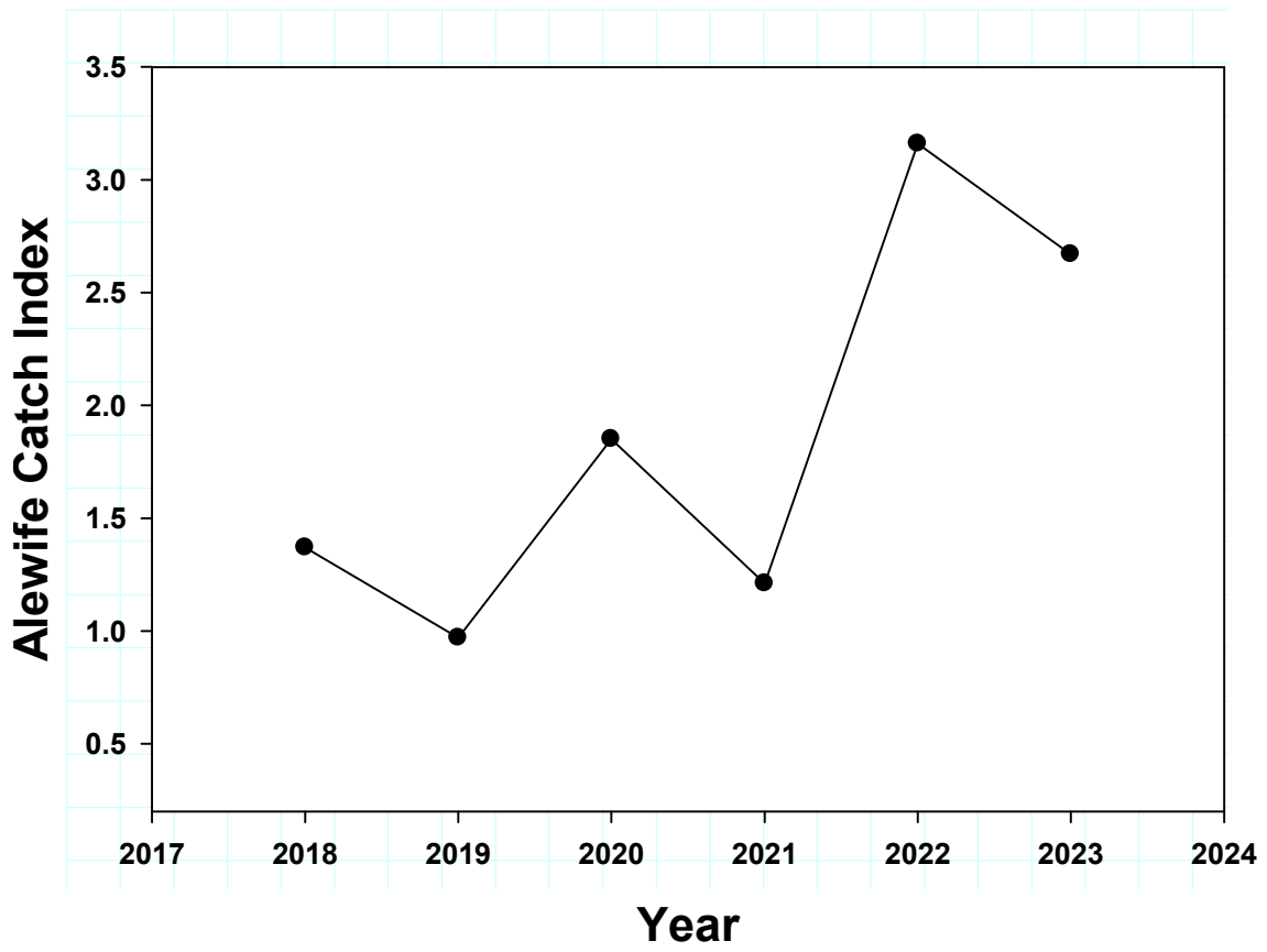
Figure 14. Recent (2018-2023) values of the catch index of female Alewife on the Rappahannock River.
