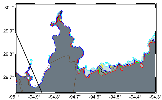
Figure S12: Ike Inundation Extents by Trinity Bay and Chambers County, TX for ADCIRC ( blue ), SWAN+ADCIRC ( cyan ), FVCOM ( red ), SWAN-FVCOM ( black ), SELFE ( green ), and WWMII+SELFE ( yellow ). The hurricane track is shown by the thick black line , and the coastline by the brown line .
