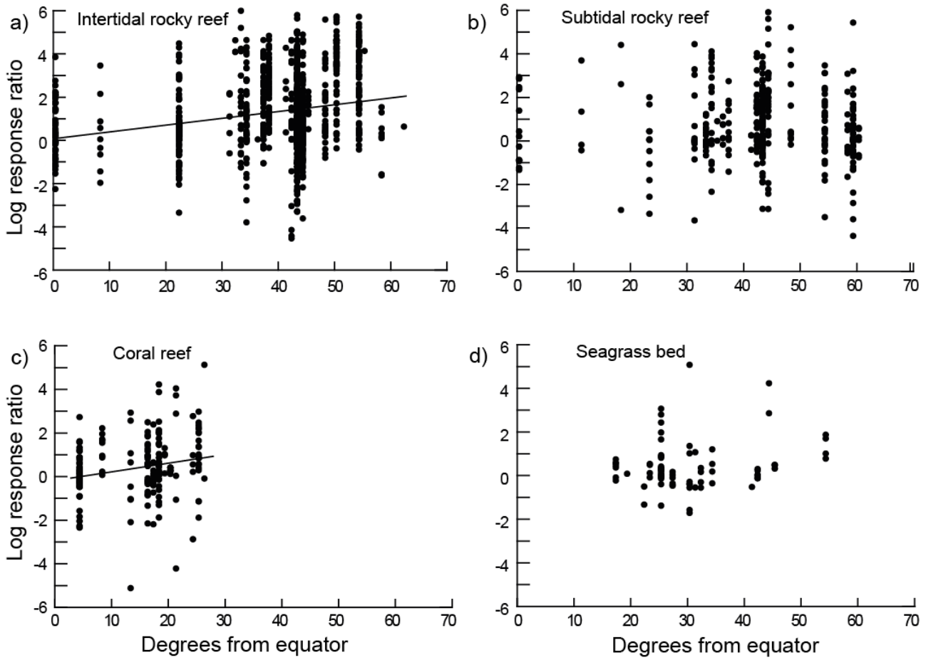
Fig. S1 Variation in the effects of excluding grazers with absolute latitude for each of the major habitat types; intertidal rocky reefs (a), subtidal rocky reefs (b), coral reefs (c) and seagrass beds (d).
