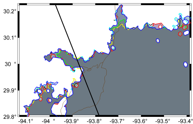
Figure S07: Rita inundation extents by Sabine Lake for ADCIRC ( blue ), SWAN+ADCIRC ( cyan ), FVCOM ( red ), SWAN-FVCOM ( black ), SELFE ( green ), and WWMII+SELFE ( yellow ). The hurricane track is shown by the thick black line , and the coastline by the brown line .
