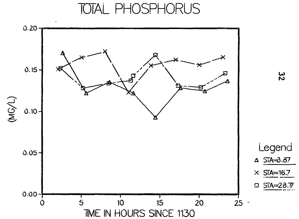
Figure 14c. Nansemond River mean concentrations at the downstream (3.87 km), mid-estuary (16.7 km), and upstream (28.77 km) stations throughout the 24-hour Intensive survey, September 27-28, 1982.
