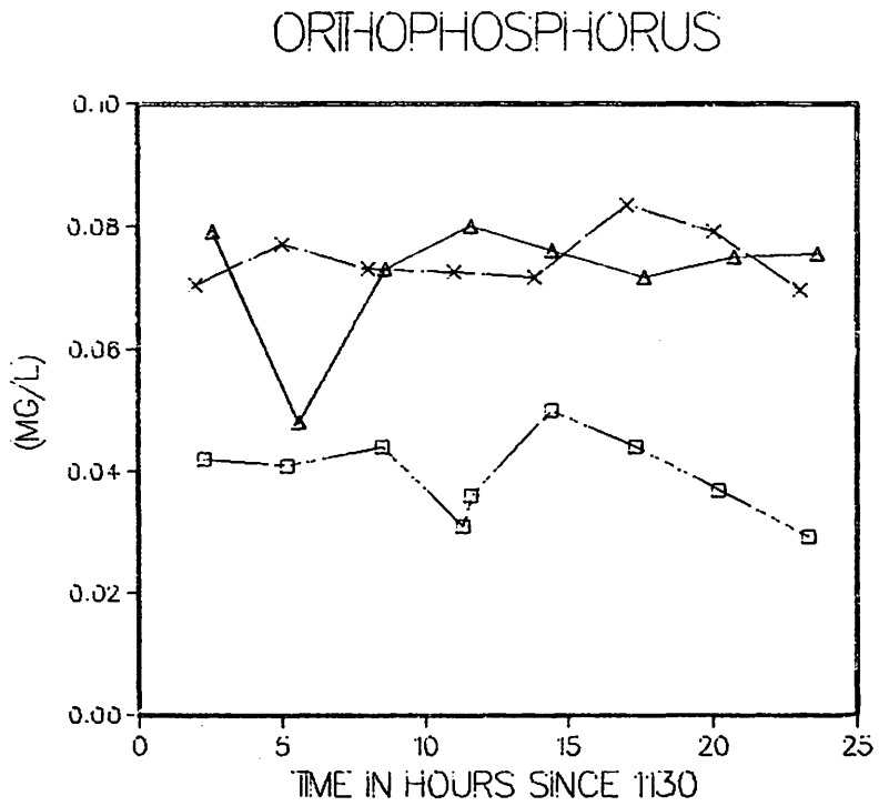
Figure 14c. Nansemond River mean concentrations at the downstream (3.87 km), mid-estuary (16.7 km), and upstream (28.77 km) stations throughout the 24-hour Intensive survey, September 27-28, 1982.
