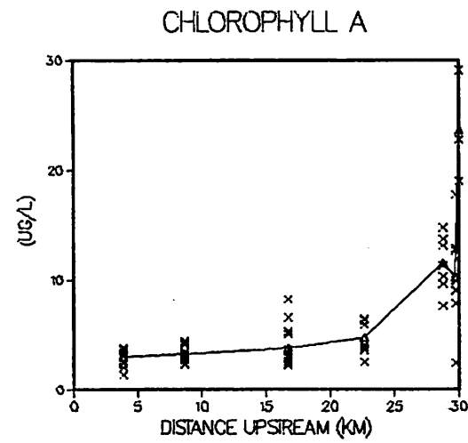
Figure 13b. Mean concentrations ( \Delta ) and values (x) during the September 27-28, 1982 Intensive survey on the Nansmond River.
