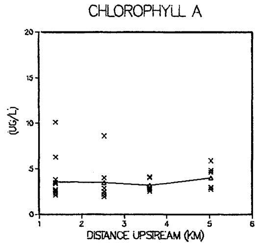
Figure 20b. Mean concentrations ( \Delta ) and values (x) during the September 27-28, 1982 Intensive survey on Chuckatuck Creek.
