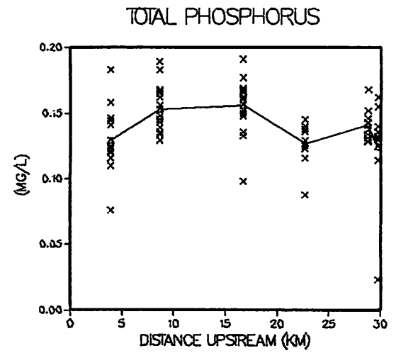
Figure 13b. Mean concentrations ( \Delta ) and values (x) during the September 27-28, 1982 Intensive survey on the Nansmond River.
