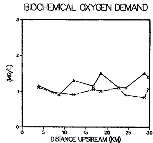
Figure 4a. March 14, 1983 high slackwater (Δ) and March 17, 1983 low slackwater (X) surveys in the Nansemond River.
