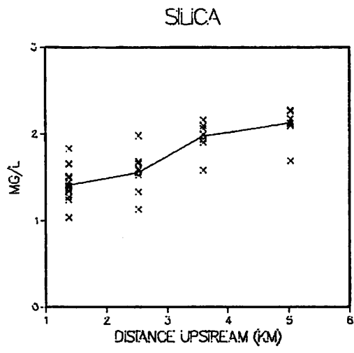
Figure 20a. Mean concentrations (Δ) and values (x) during the September 27-28, 1982 Intensive survey on Chuckatuck Creek.
