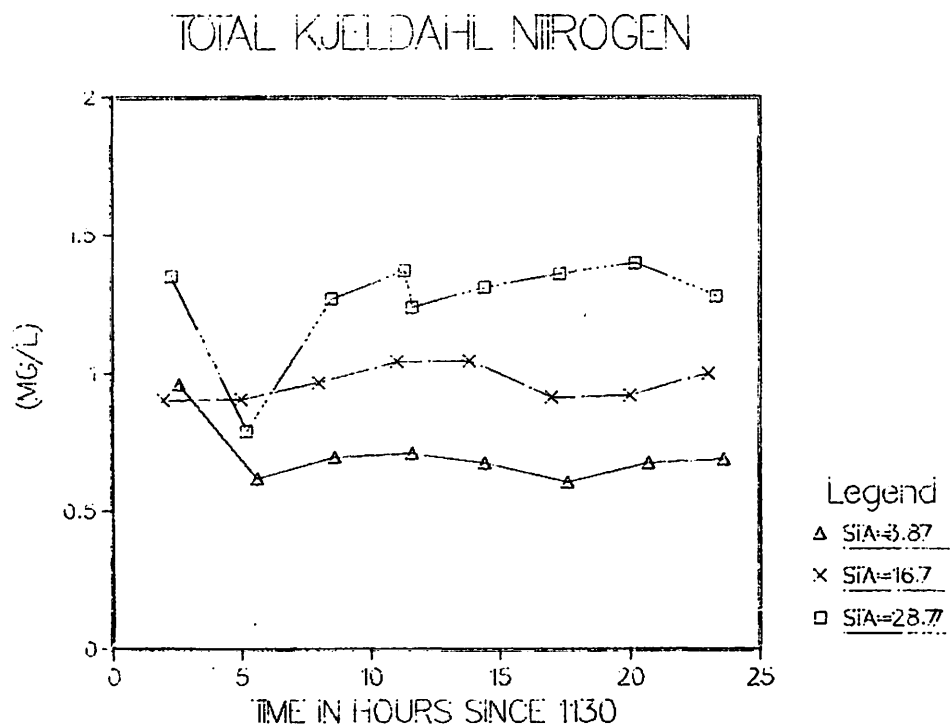
Figure 14d. Nansemond River mean concentrations at the downstream (3.87 km), mid-estuary (16.7 km), and upstream (28.77 km) stations throughout the 24-hour Intensive survey, September 27-28, 1982.
