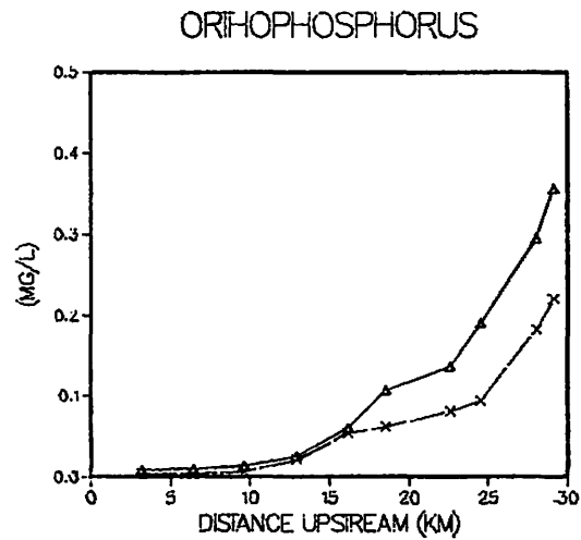
Figure A-4. January 5, 1967 (Δ) and February 1, 1967 (X) surveys in the Nansemond River.
