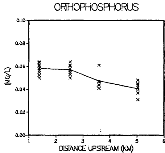
Figure 20b. Mean concentrations ( \Delta ) and values (x) during the September 27-28, 1982 Intensive survey on Chuckatuck Creek.
