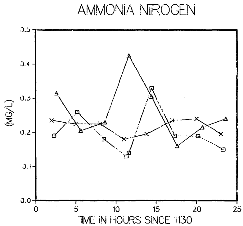
Figure 14b. Nansemond River mean concentrations at the downstream (3.87 km), mid-estuary (16.7 km), and upstream (28.77 km) stations throughout the 24-hour Intensive survey, September 27-28, 1982.
