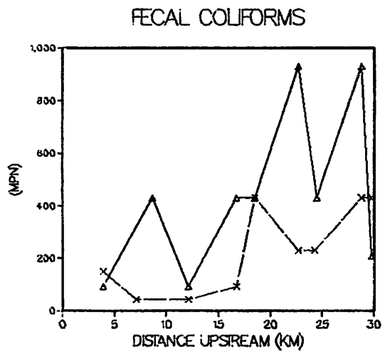
Figure 4a. March 14, 1983 high slackwater (Δ) and March 17, 1983 low slackwater (X) surveys in the Nansemond River.
