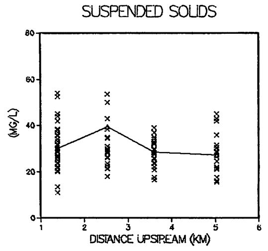
Figure 20a. Mean concentrations (Δ) and values (x) during the September 27-28, 1982 Intensive survey on Chuckatuck Creek.
