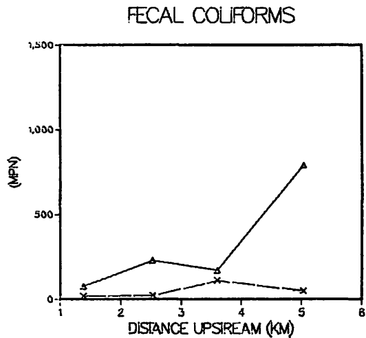
Figure 17a. July 15, 1982 low slackwater (Δ) and July 19, 1982 high slackwater (X) surveys in Chuckatuck Creek. The first survey was conducted under "wet" conditions, the latter under "dry" conditions.
