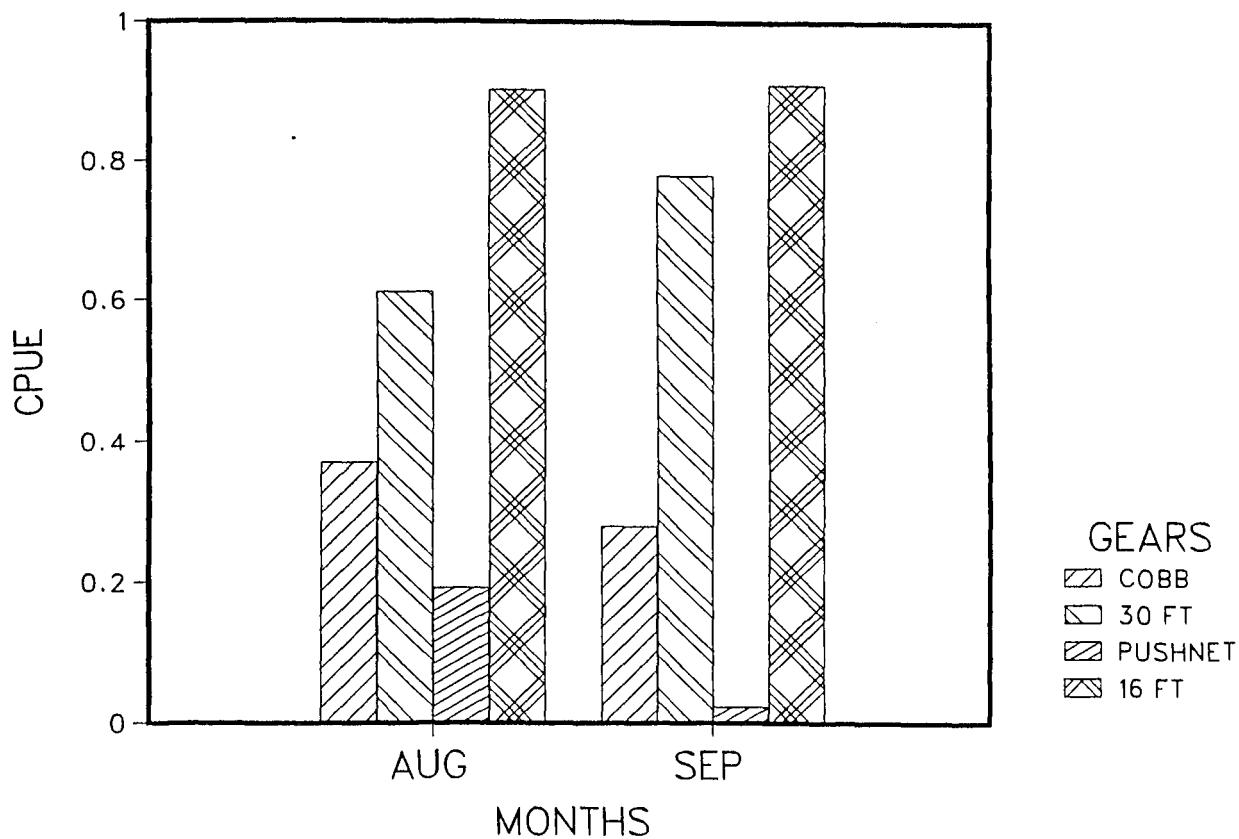
Figure 16. Mean catch per 5 min. tow by sampling gear of striped bass taken during 1978 VIMS comparison studies.
