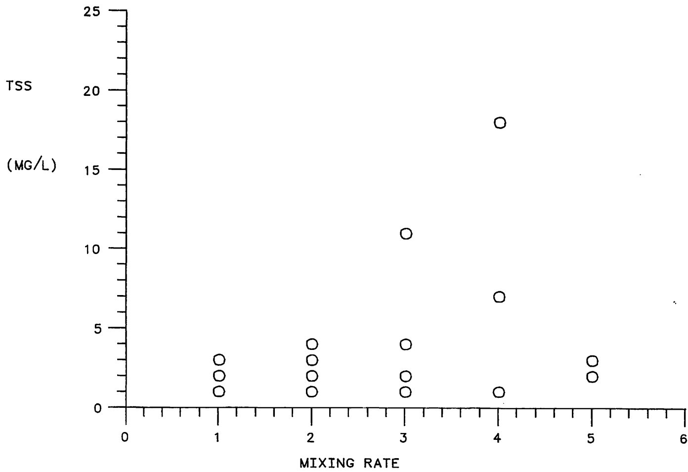
Figure 5. Total suspended solids vs. mixing rate.
