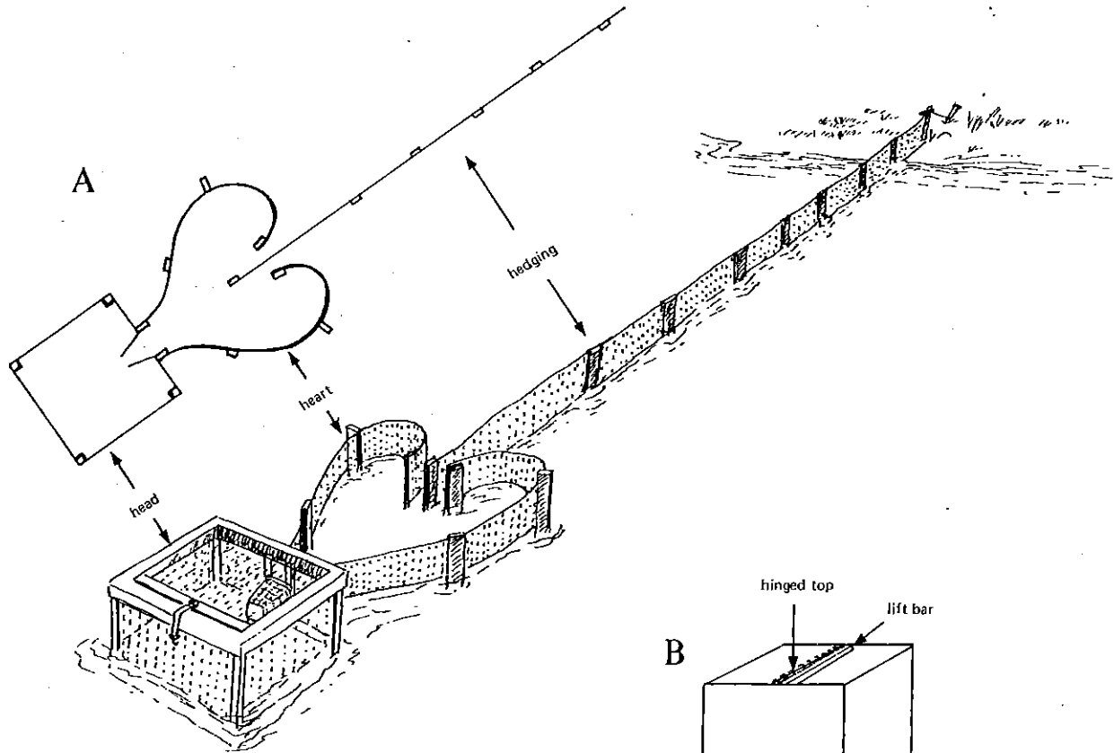
FIGURE 8. (A) A typical peeler pound net showing the basic parts and usual placement relative to the shoreline.
