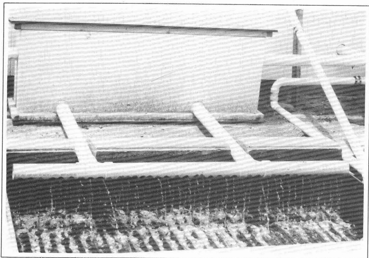
FIGURE 26. Corrugated fiberglass roofing material is used within the biological filter to evenly distribute incoming water over the filter media. The use of a "spray manifold" also increases water distribution, as well as reoxygenation of the water. The white box in this picture contains a mechanical filter to pre-screen water before it enters the biological filter.
