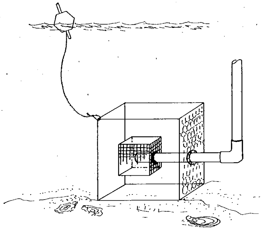
FIGURE 16. Construction details for a two-box screened water intake. The smaller, inner box should be constructed of small mesh wire (1/4"). The larger outer box should be larger mesh (1"). A buoyed line is attached to allow for raising the screened intake for periodic cleaning.
