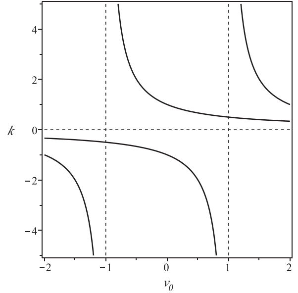
FIG. 1. A plot of the surface D' = 0 , where D' is defined in (2), using \omega = 1 and c_s = 1 . The plot is shown in terms of k and v_0 . To guide the eye, we have also plotted the lines v_0 = \pm 1 and k = 0 (all three of these lines are dashed). The avoided crossings, where v_0^2 = c_s^2 = 1 , are clear.
