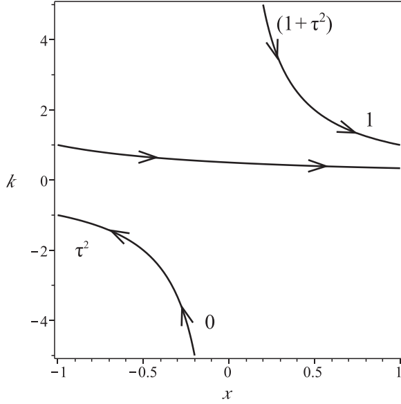
FIG. 2. A plot of the surface D=0 , now restricted to the region around the resonance at v_0 = +c_s = 1 , assuming a linear velocity profile of the form v_0(x) = c_s(0)(1 + \frac{x}{L}) = (1+x) , where we have set c_s(0) = 1 , and L = 1 . Note that this plot uses x as the horizontal axis. An avoided crossing type of behavior is present at the resonance, where \lambda_-(x, k) = 0 , but there is an additional branch where \lambda_+(x, k) = 0 is present as well, so this is not tunneling of the standard type. See text for details.
