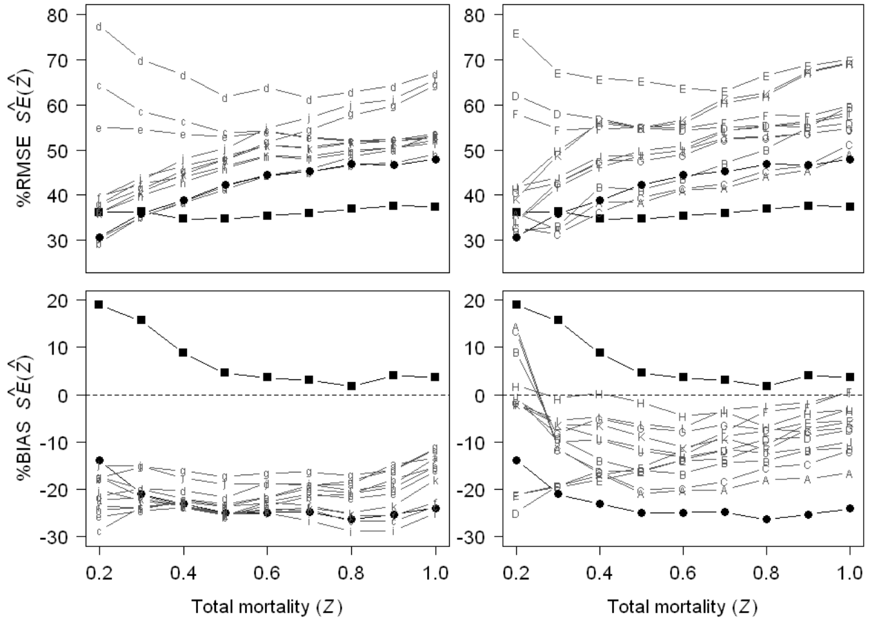
Figure 45. Performance of the Chapman-Robson Peak Plus variance estimator with correction for overdispersion ( \blacksquare ), and the RG Peak weighted regression variance estimator ( \bullet ) in terms of %RMSE ( top ) and %BIAS ( bottom ). In the left column, highlighted variance estimators are plotted against all other simulated weighted regression variance estimators (a = RG Peak plus, b = R1 Peak, c = R1 Peak plus, d = R1 z-test, e = R1' Peak, f = R1' Peak plus, g = R1' z-test, h = R1'' Peak, i = R1'' Peak plus, j = R1'' z-test). In the right column, the preferred highlighted variance estimators are plotted against all other simulated unweighted regression variance estimators (A = RG Peak, B = RG Peak plus, C = RG z-test, D = R1 Peak, E = R1 Peak plus, F = R1 z-test, G = R1' Peak, H = R1' Peak plus, I = R1' z-test, J = R1'' Peak, K = R1'' Peak plus, and L = R1'' z-test). Simulation conditions were M = 0.2 \text{ year}^{-1} , steep selectivity/partial recruitment curves, N = 200 , \sigma = 0.6 where M is the instantaneous natural mortality rate, N is the sample size, and \sigma is the total error.
