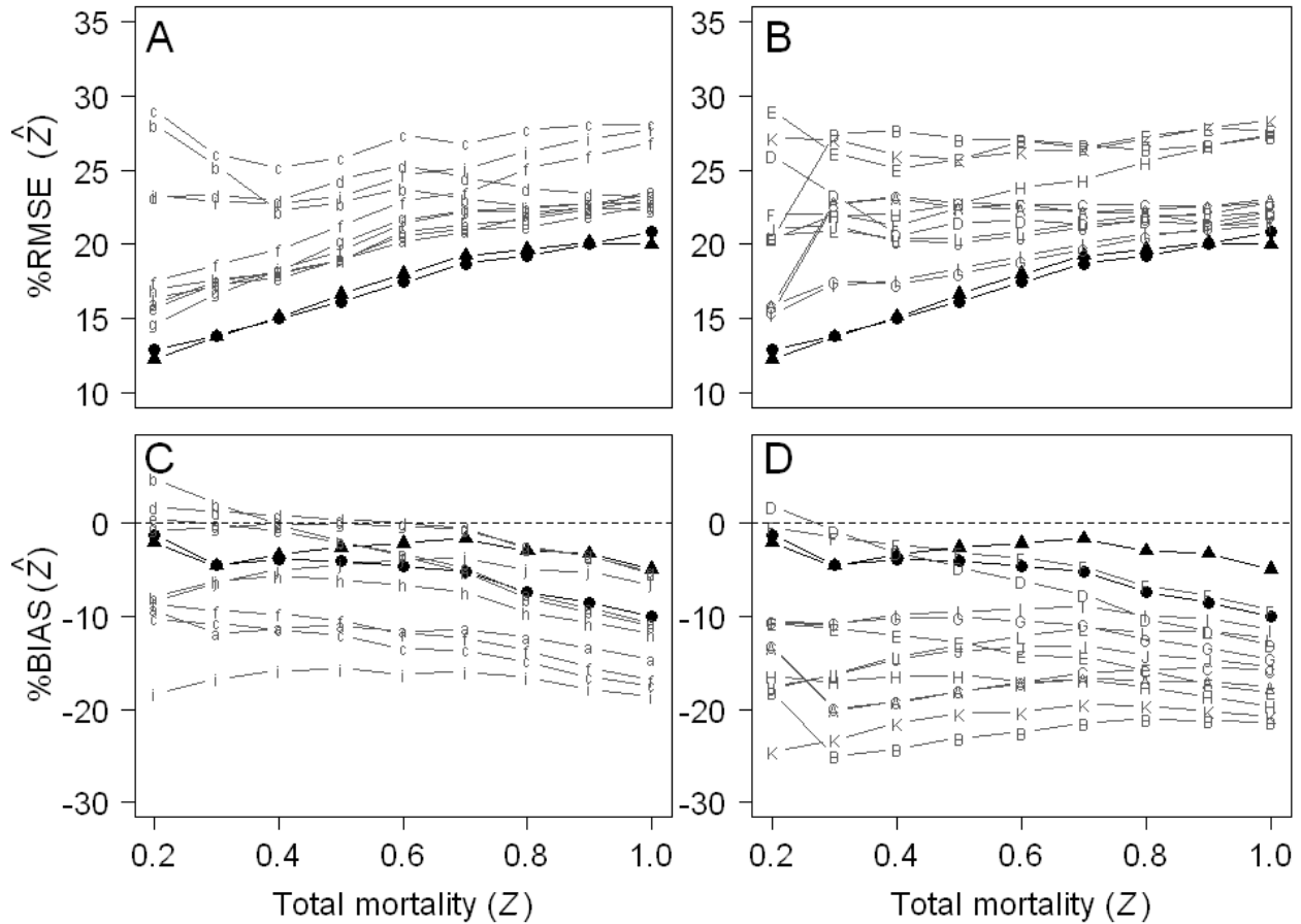
Figure 20. %BIAS ( bottom ) and %RMSE ( top ) of various mortality estimators as a function of total mortality rate ( Z ). Panels A and C: the preferred weighted regression methods (RG Peak \bullet and RG z-test \blacktriangle ) compared to all other simulated weighted regressions (a = RG Peak plus, b = R1 Peak, c = R1 Peak plus, d = R1 z-test, e = R1' Peak, f = R1' Peak plus, g = R1' z-test, h = R1'' Peak, i = R1'' Peak plus, j = R1'' z-test). Simulation conditions were M = 0.2 year -1 , gradual selectivity/partial recruitment curves, N = 600 , \sigma = 0.6 where M is the instantaneous natural mortality rate, N is the sample size, and \sigma is the total error. Panels B and D: the preferred weighted regressions (as indicated above) compared to all simulated unweighted regressions (A = RG Peak, B = RG Peak plus, C = RG z-test, D = R1 Peak, E = R1 Peak plus, F = R1 z-test, G = R1' Peak, H = R1' Peak plus, I = R1' z-test, J = R1'' Peak, K = R1'' Peak plus, and L = R1'' z-test). Simulation conditions were the same as in Panels A and C.
