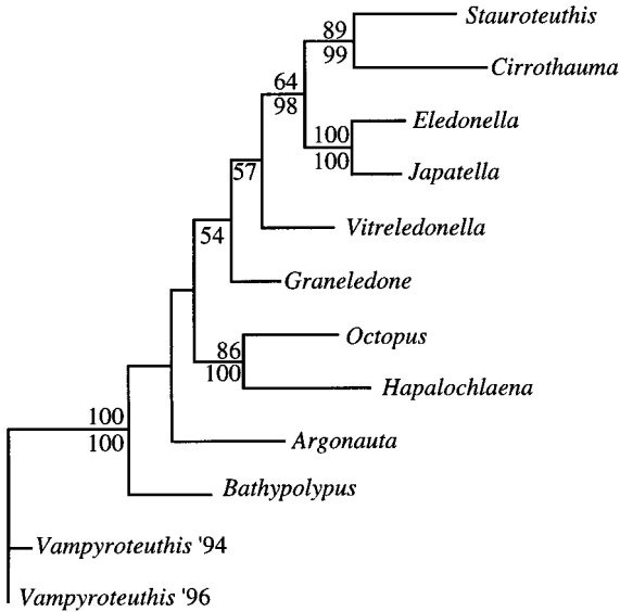
Figure 3. Most parsimonious tree produced from phylogenetic analysis of octopod COI nucleotide sequences using the Vampyromorpha as outgroup. Analysis of the unweighted data (TL = 692, CI = 0.529, RI = 0.468, bootstrap indices > 50% above nodes) and the RCI-weighted data (TL = 190, 139), CI = 0.751, RI = 0.710, bootstrap indices > 50% below nodes) resulted in an identical tree topology.
