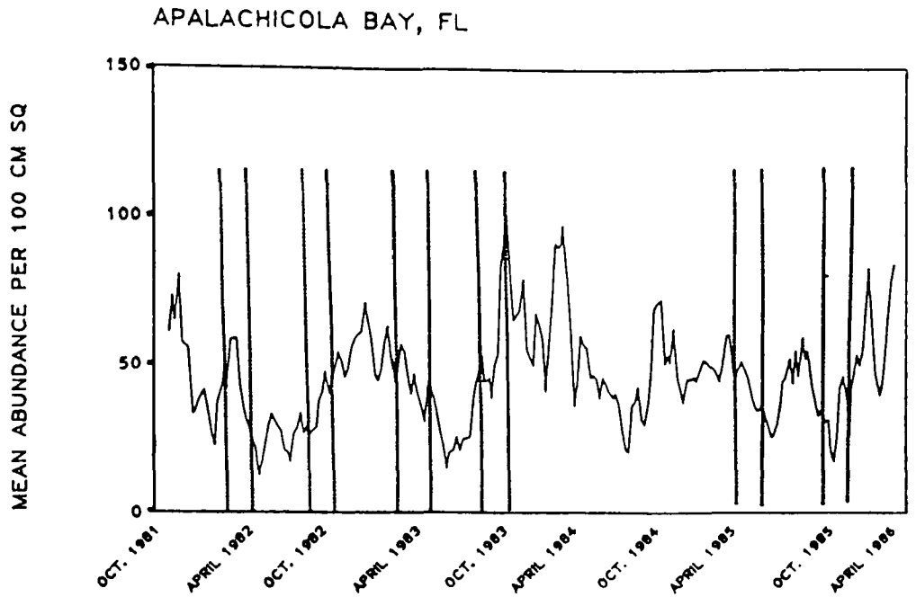
FIGURE 2 - MEAN ABUNDANCE IN WEEKLY SAMPLES FROM 1981 - 1986. Vertical lines indicate test dates.
