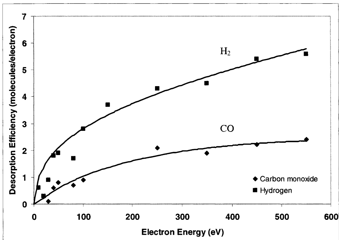
FIGURE 6.7 The desorption efficiency of CO and H 2 increase as electron energy increases, with hydrogen being the most significant gas desorbed.[92]
