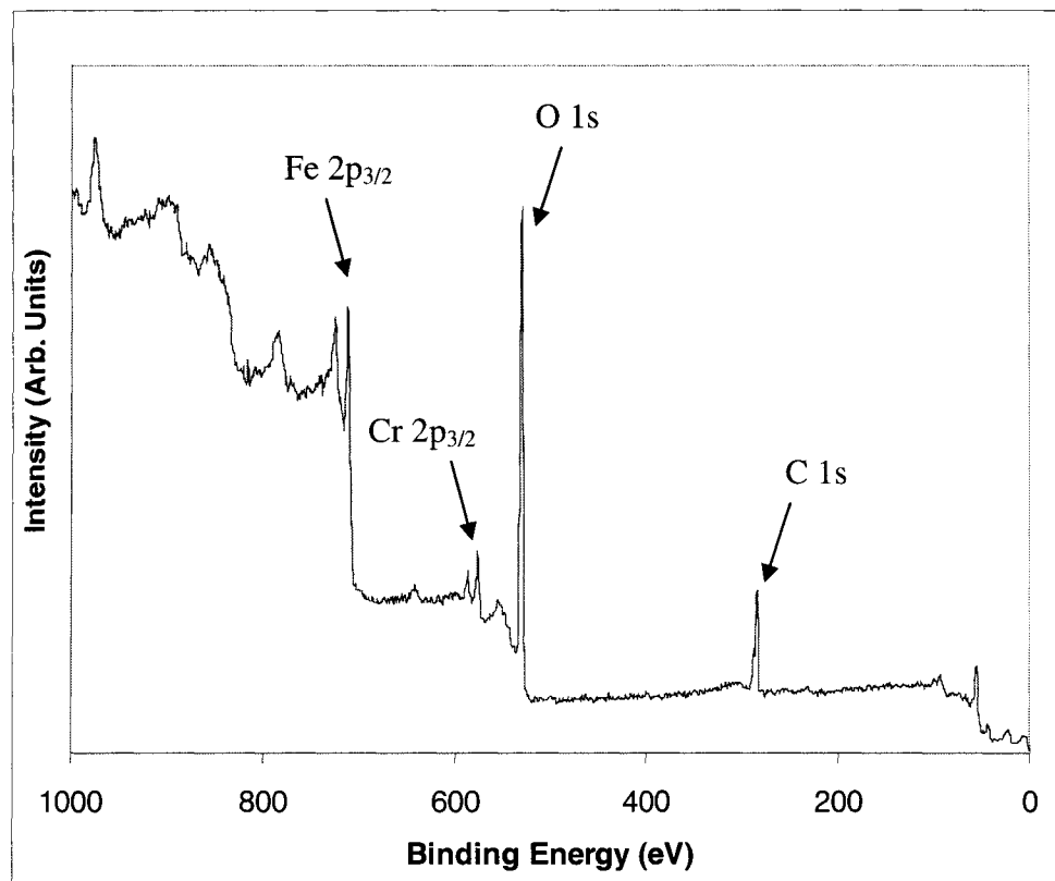
FIGURE 3.4 An XPS survey spectrum of stainless steel.
