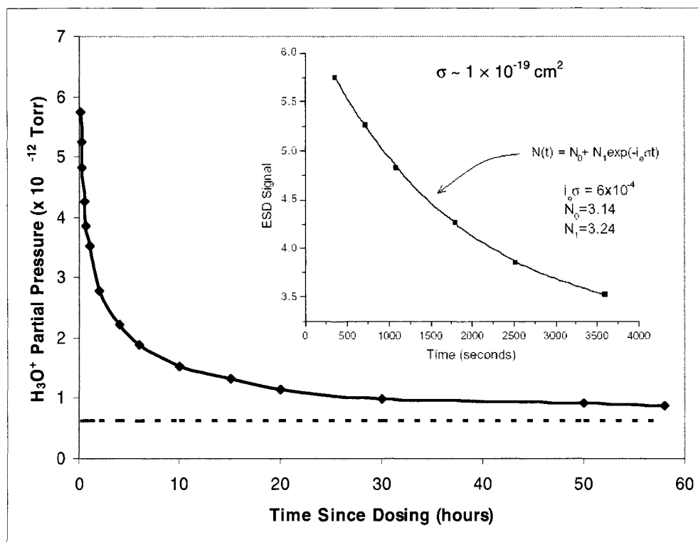
FIGURE 5.6 After hydrogen is allowed to saturate the system components for 8 hours at 1.0 \times 10^{-6} Torr, the signal at mass 19 increases by 10\times from its pre-dose value (dashed line). The signal then begins to decrease over time. Inset is the first six points from which the ESD cross section \sigma \sim 1 \times 10^{-19} \text{ cm}^2 is estimated.[11]
