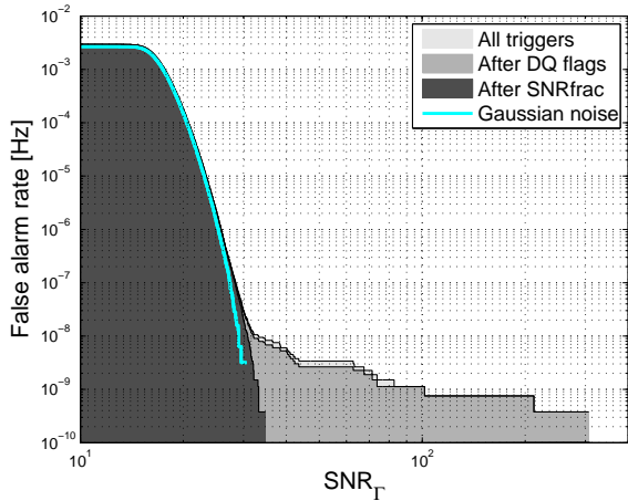
Figure 2: The false alarm rate is shown as a function of the trigger \text{SNR}_T , for 100 time-shifts of data from the S5 science run. Distributions are shown before and after applying the post-processing cuts. Here, \text{SNRfrac} refers to a post-processing cut based on how a trigger’s power is distributed in time (described further in Section IV C). Also shown is the FAR distribution generated by a Monte Carlo simulation assuming Gaussian detector noise. Recall that this is an energy SNR, rather than an amplitude SNR.
