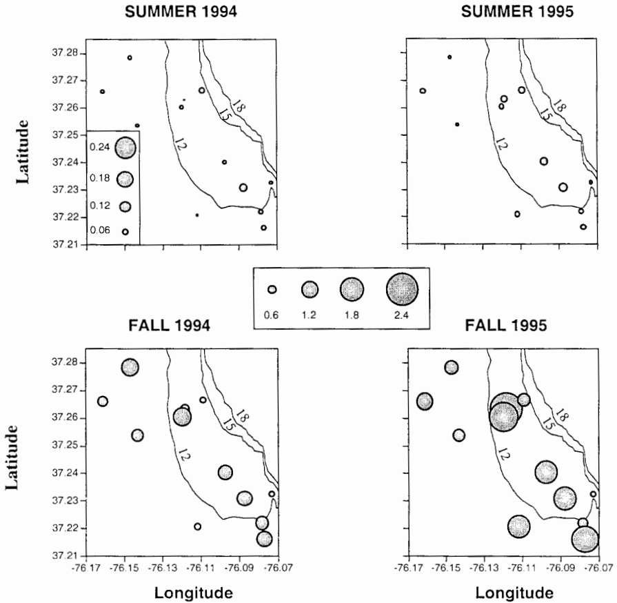
Figure 5. Total station ash free dry weight (g AFDW 0.06 \text{ m}^{-2} ). Data are graphed as area bubble plots with stations arranged by latitude and longitude, separated by year, and grouped by season. Note scale changes; Summer 1994 is an order of magnitude less. Solid lines are depth contours in meters.
