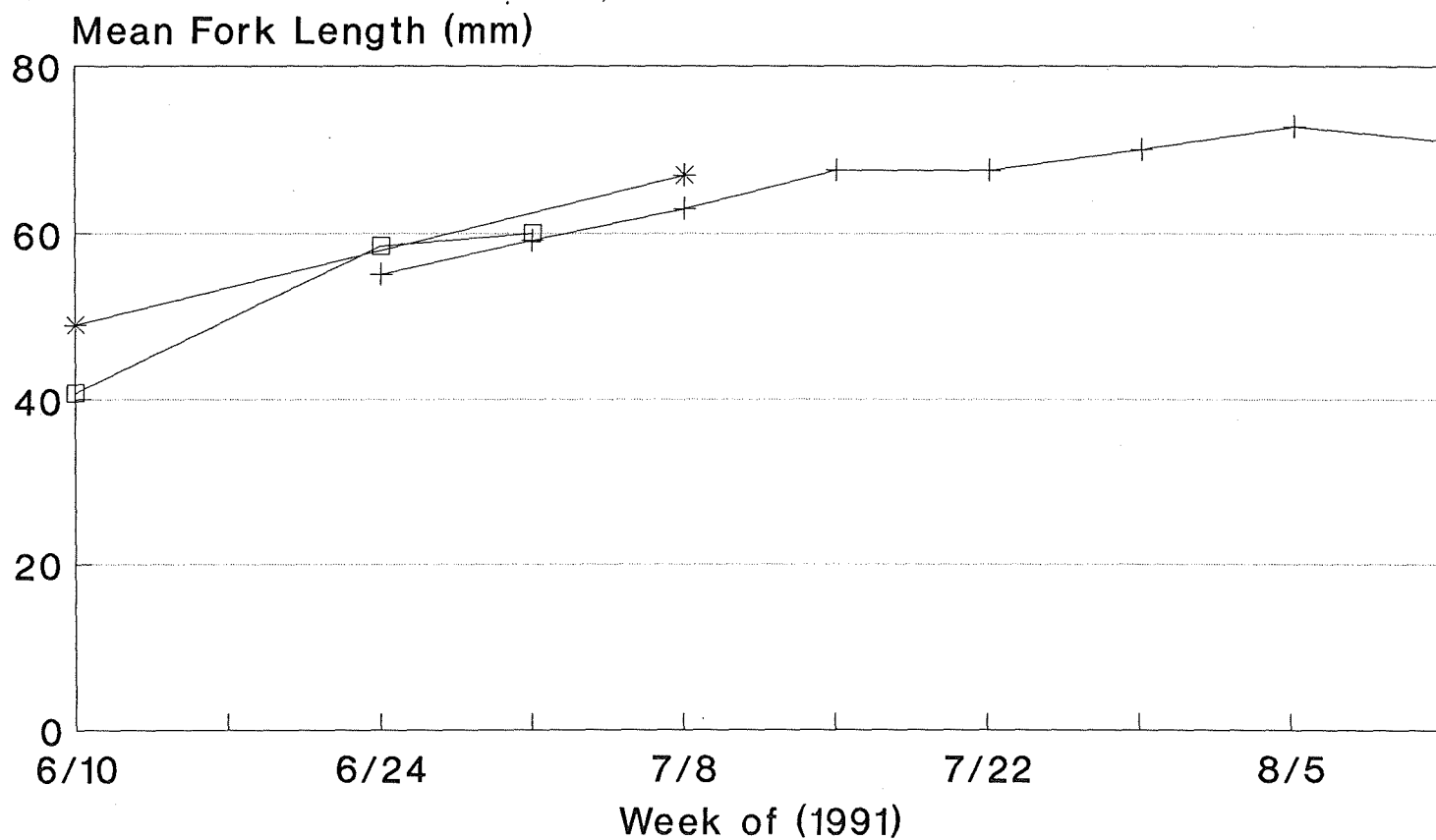
Figure 10 - Apparent Growth Curve Alewife (All Rivers)
