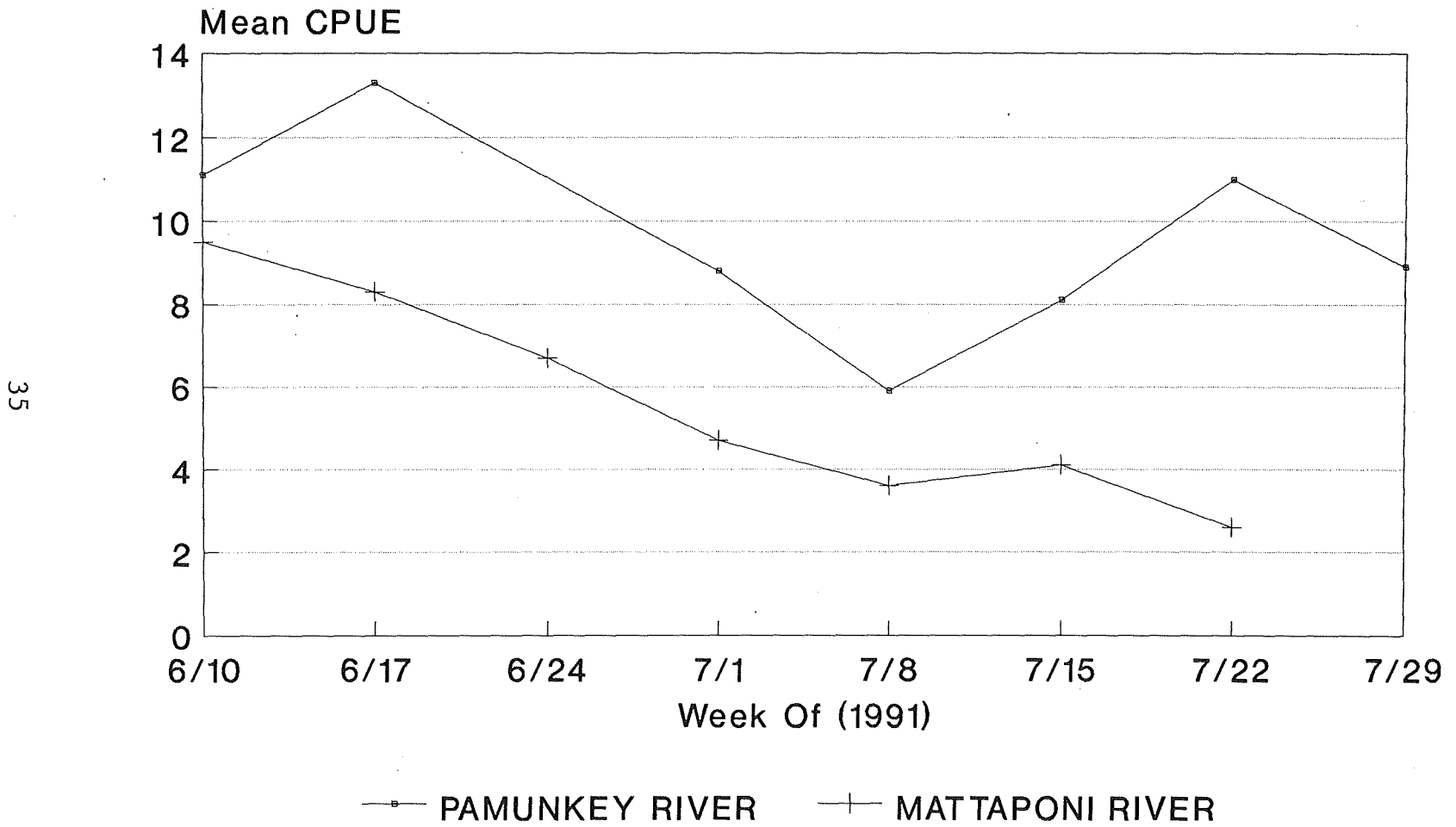
Figure 4 - Juvenile Alosa Catch Curve Blueback Herring (Pamunkey-Mattaponi R.)
